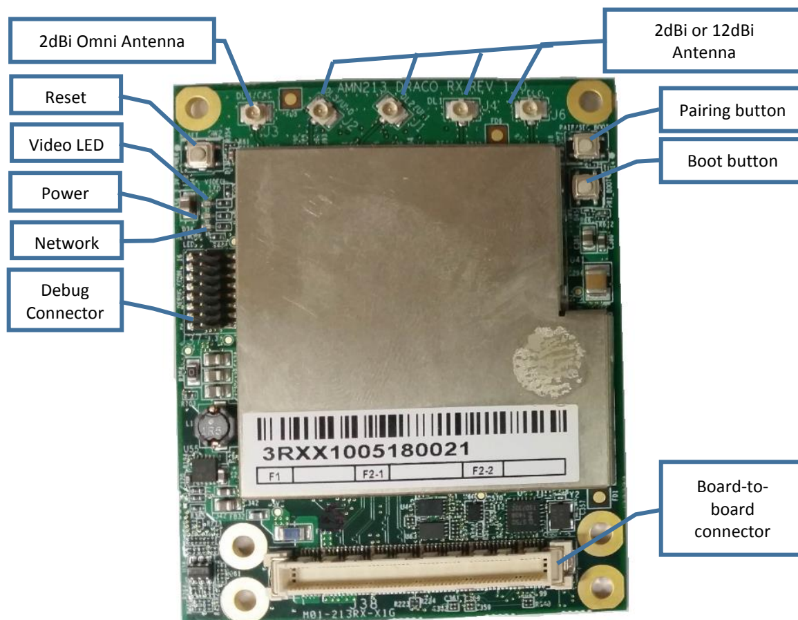
Figure 2 – AMN42012 top view
