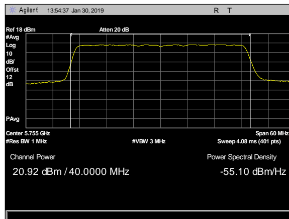
Plot 11. Output Power, 2dBi & 5dBi 4x4, 5755MHz, c4
