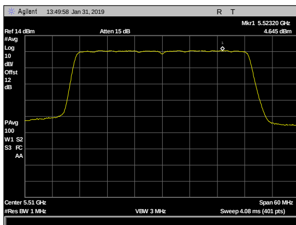
Plot 103. Power Spectral Density, 2dBi, 2x2, 5510MHz c2
