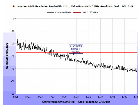
Plot 234. Radiated Band Edge, -27dBm, 5725, BW40M, CF5670MHz, 2x2, 5dBi
