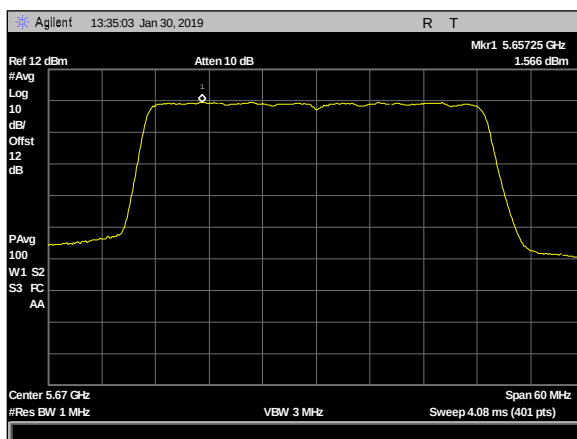
Plot 139. Power Spectral Density, 5dBi, 4x4, 5670MHz c4
