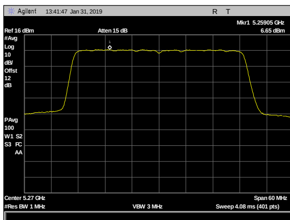
Plot 94. Power Spectral Density, 2dBi, 2x2, 5270MHz c1
