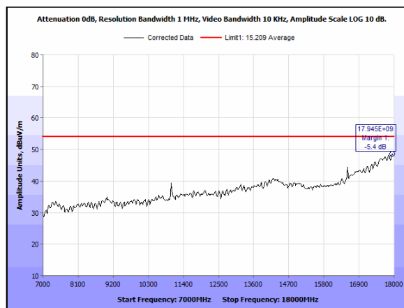
Plot 149. Radiated Emissions, Average, 2x2, 5dBi, 5510, 7-18GHz
