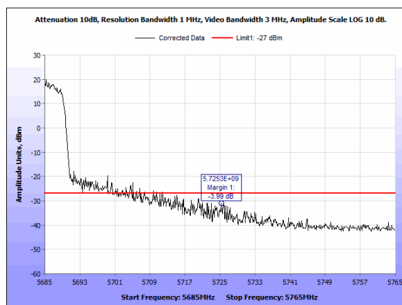
Plot 237. Radiated Band Edge, -27dBm, 5725, BW40M, CF5670MHz, 4x4, 5dBi
