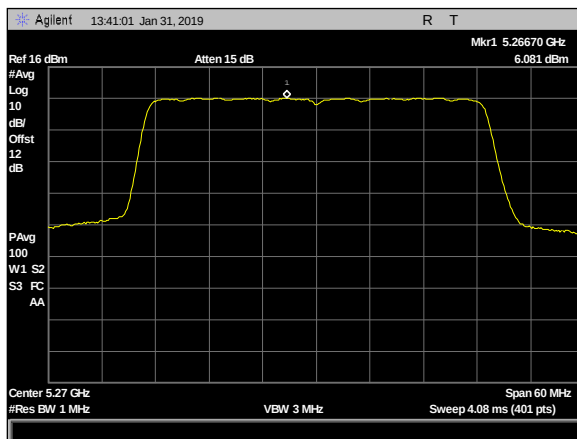
Plot 95. Power Spectral Density, 2dBi, 2x2, 5270MHz c2
