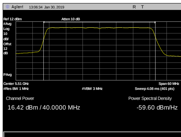
Plot 45. Output Power, 5dBi, 4x4, 5510MHz c4
