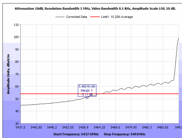
Plot 241. Radiated Band Edge, Average, 5460, BW40M, CF5510MHz, 2x2, 2dBi
