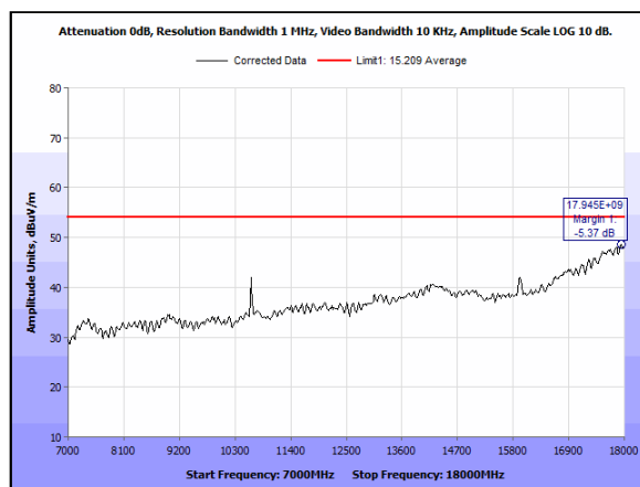
Plot 147. Radiated Emissions, Average, 2x2, 5dBi, 5310, 7-18GHz
