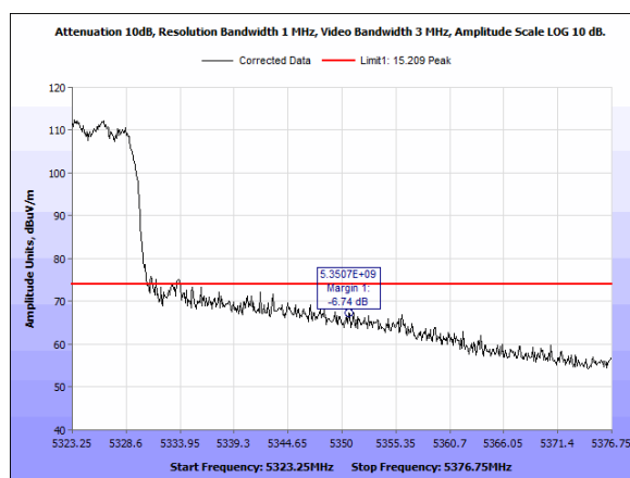
Plot 227. Radiated Band Edge, Peak, 5350, BW40M, CF5310MHz, 2x2, 2dBi
