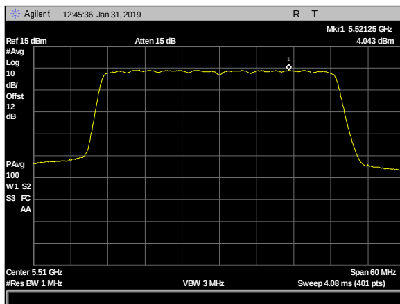
Plot 104. Power Spectral Density, 5dBi, 2x2, 5510MHz c1
