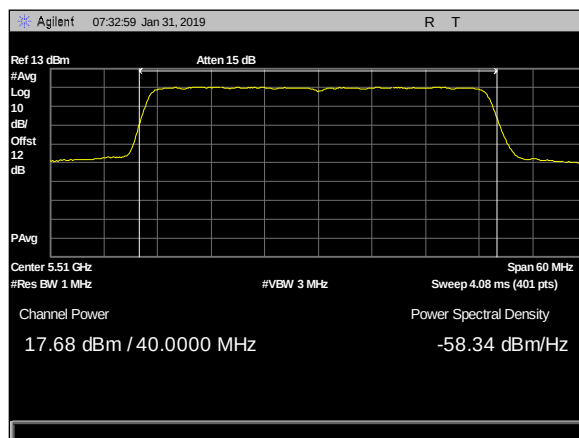
Plot 34. Output Power, 2dBi 4x4, 5510MHz c1
