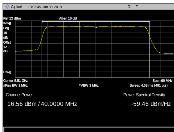
Plot 44. Output Power, 5dBi, 4x4, 5510MHz c3
