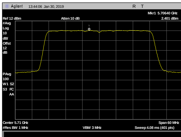
Plot 140. Power Spectral Density, 2dBi & 5dBi, 4x4, 5710MHz c1
