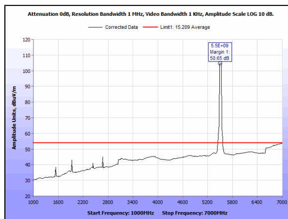
Plot 148, Radiated Emissions, Average, 2x2, 5dBi, 5510, 1-7GHz
