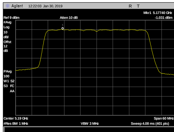
Plot 42. Power Spectral Density, 5dBi 4x4 - 5190MHz - c3
