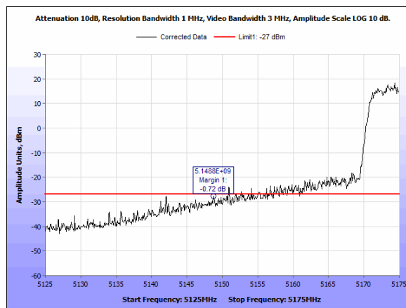
Plot 89. Radiated Bandedge, -27dBm, 5150, BW40M, CF5190MHz, 4x4, 5dBi
