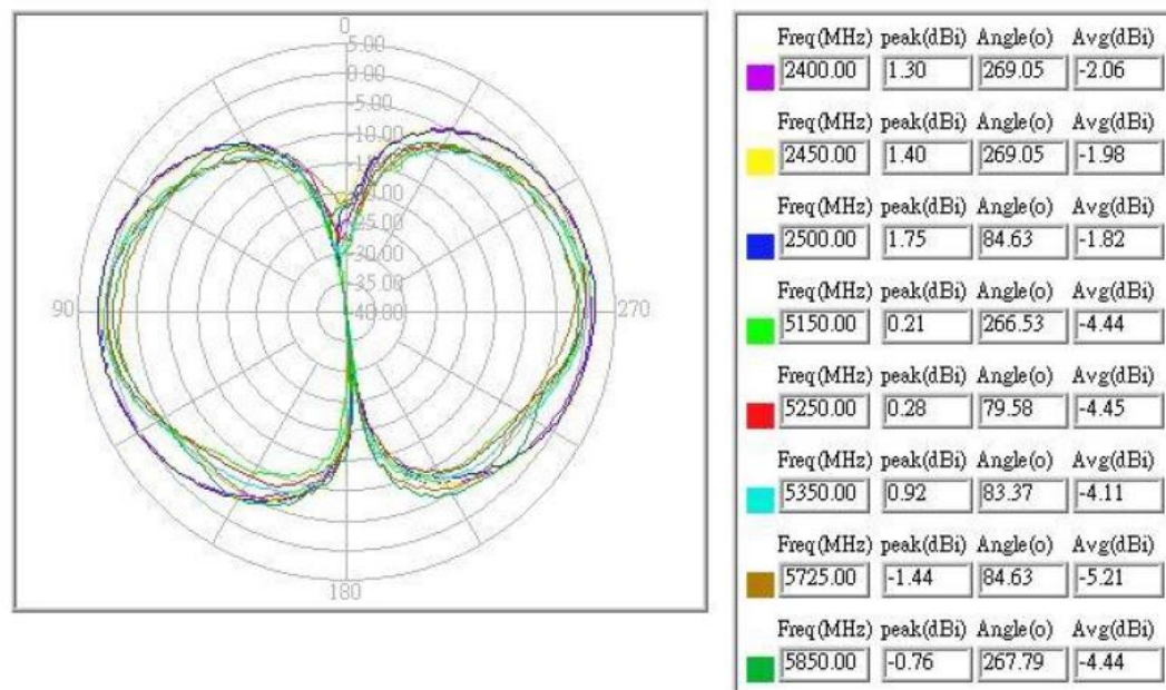
Figure 2. 2dBi Gain Antenna: Elevation Antenna Pattern
