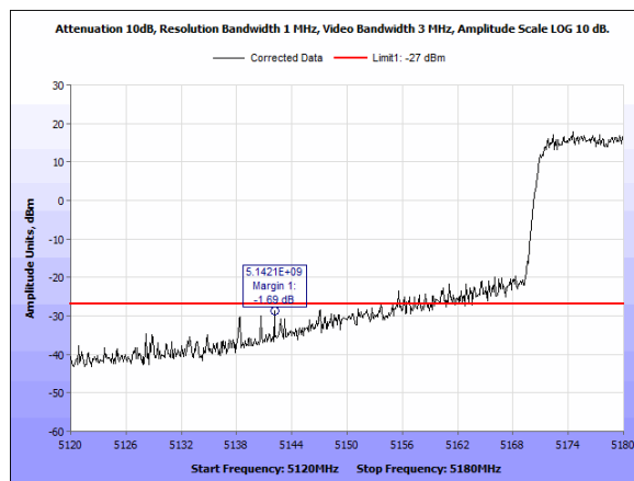
Plot 88. Radiated Bandedge, -27dBm, 5150, BW40M, CF5190MHz, 4x4, 2dBi
