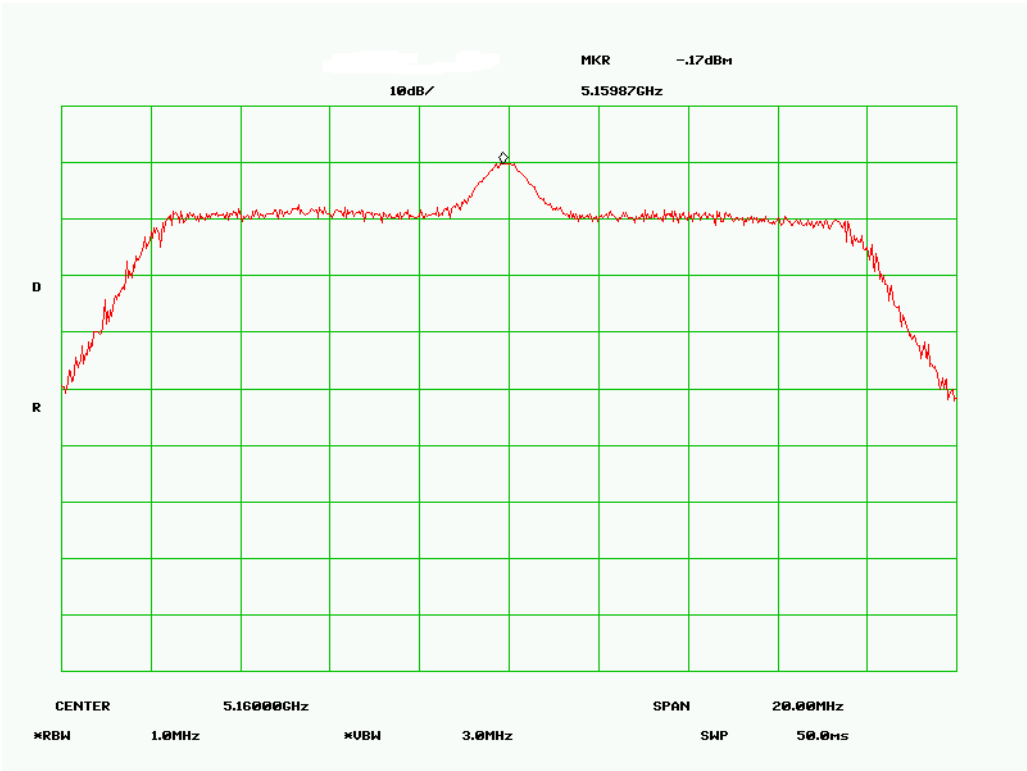
PPSD Low Channel ( )
