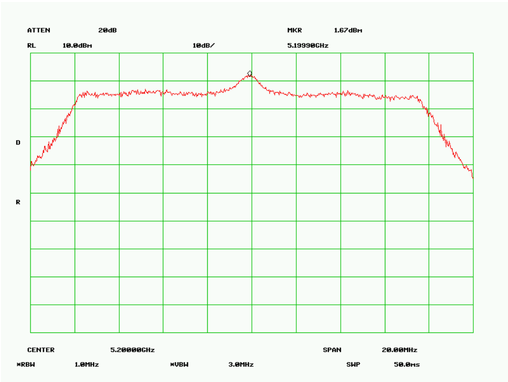
PPSD Mid Channel ( )
