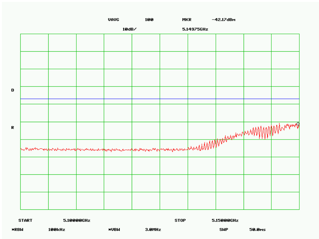
Low Channel -3 (10dB should be added to Measured Emissions)
