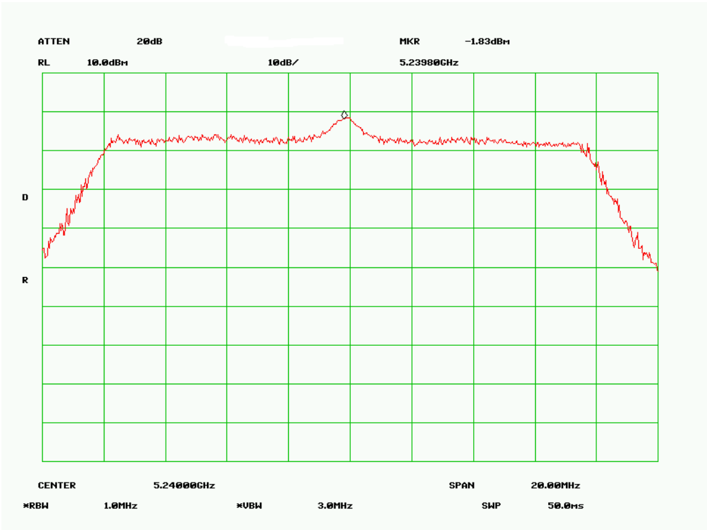
PPSD High Channel ()
