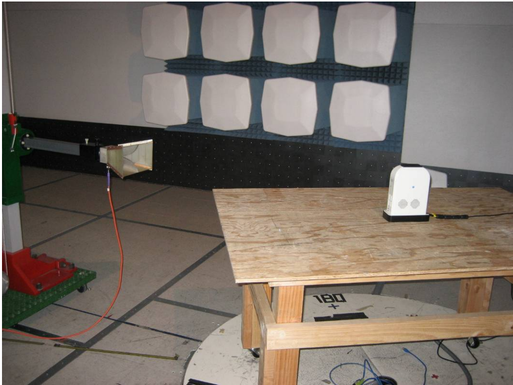
Radiated Emission Test Setup Photo ( > 1\text{GHz} )
