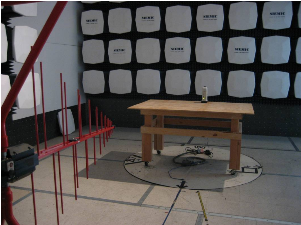
Radiated Emission Test Setup Photo (< 1GHz)
