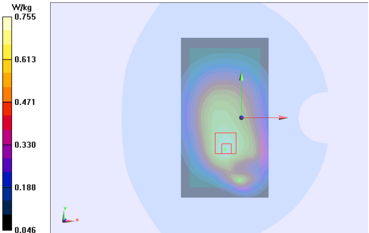
Figure 19 Body, Back Side, GSM 850 GPRS (4Txslots) Channel 190
