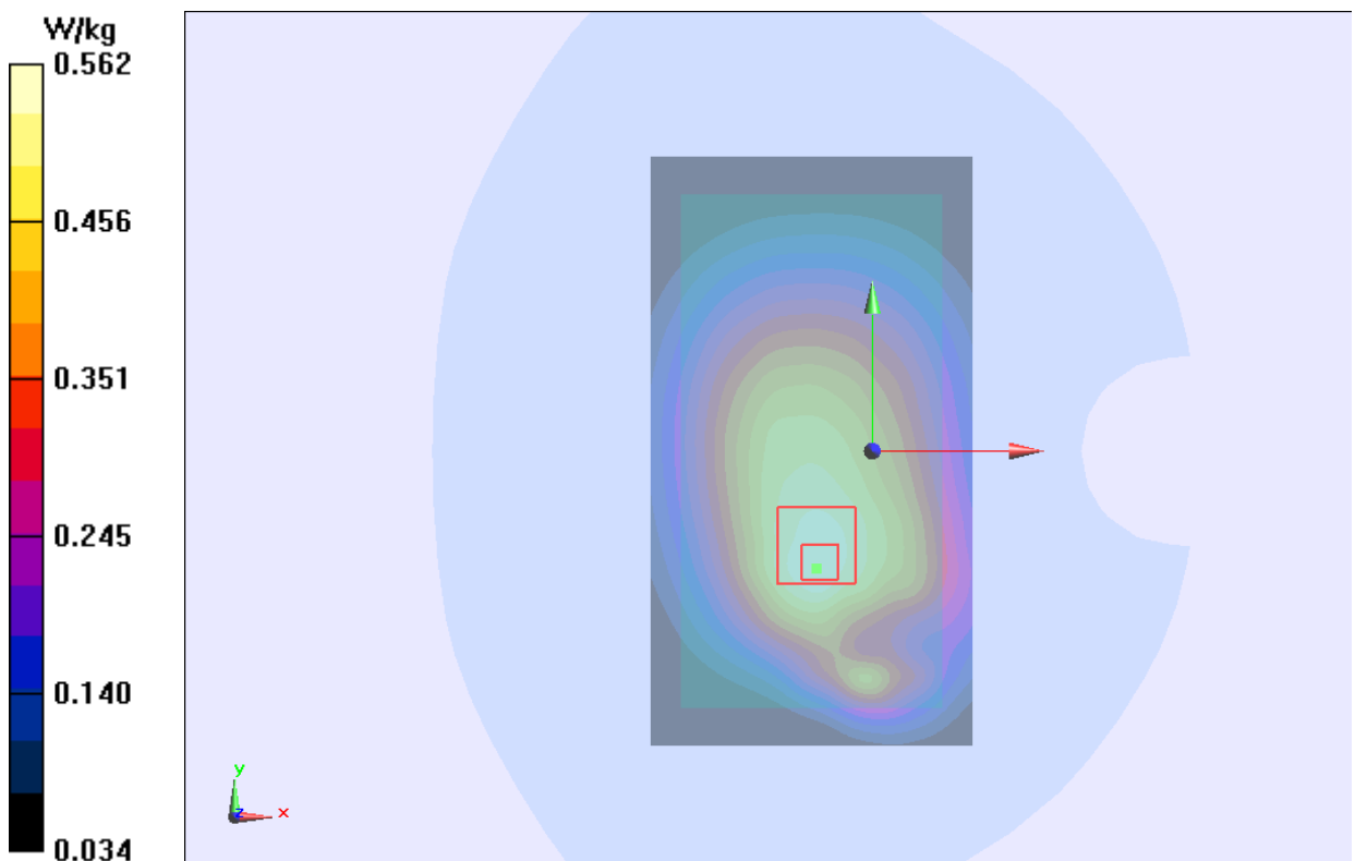
Figure 20 Body, Back Side, GSM 850 GPRS (4Txslots) Channel 128
