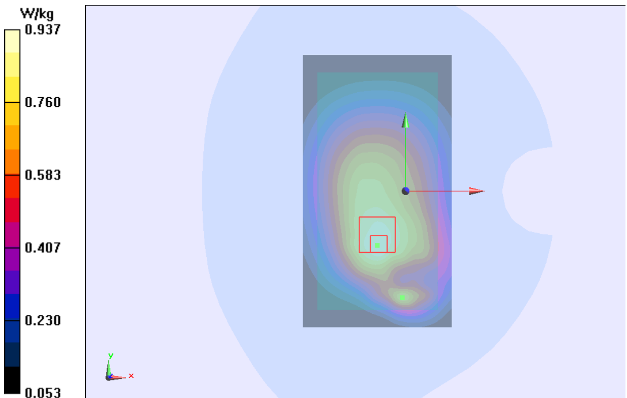
Figure 18 Body, Back Side, GSM 850 GPRS (4Txslots) Channel 251
