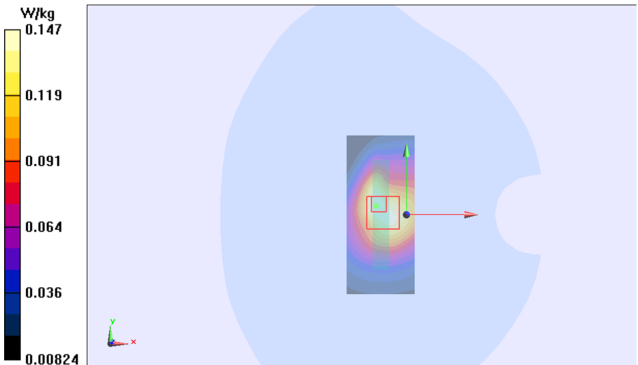
Figure 24 Body, Bottom Edge, GSM 850 GPRS (4Txslots)annel 190
