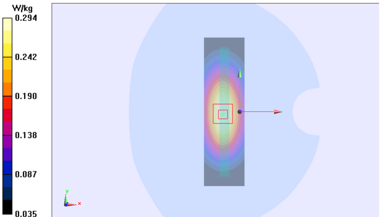
Figure 23 Body, Right Edge, GSM 850 GPRS (4Txslots)Channel 190
