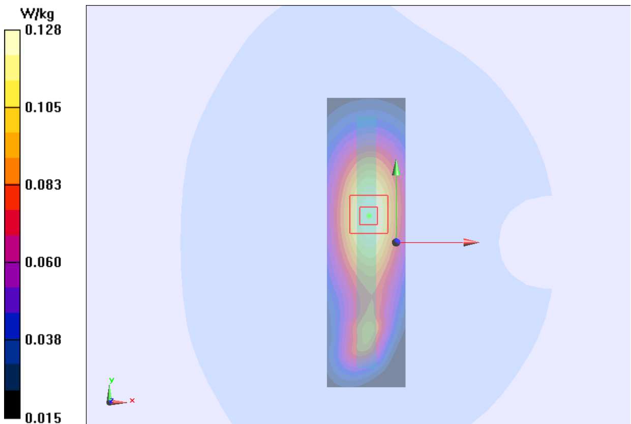
Figure 22 Body, Left Edge, GSM 850 GPRS (4Txslots)Channel 190
