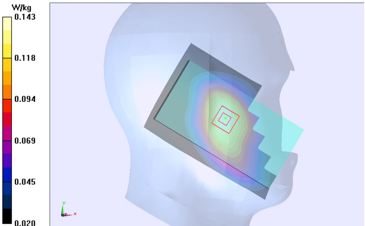
Figure 13 Left Hand Touch Cheek GSM 850 Channel 190
