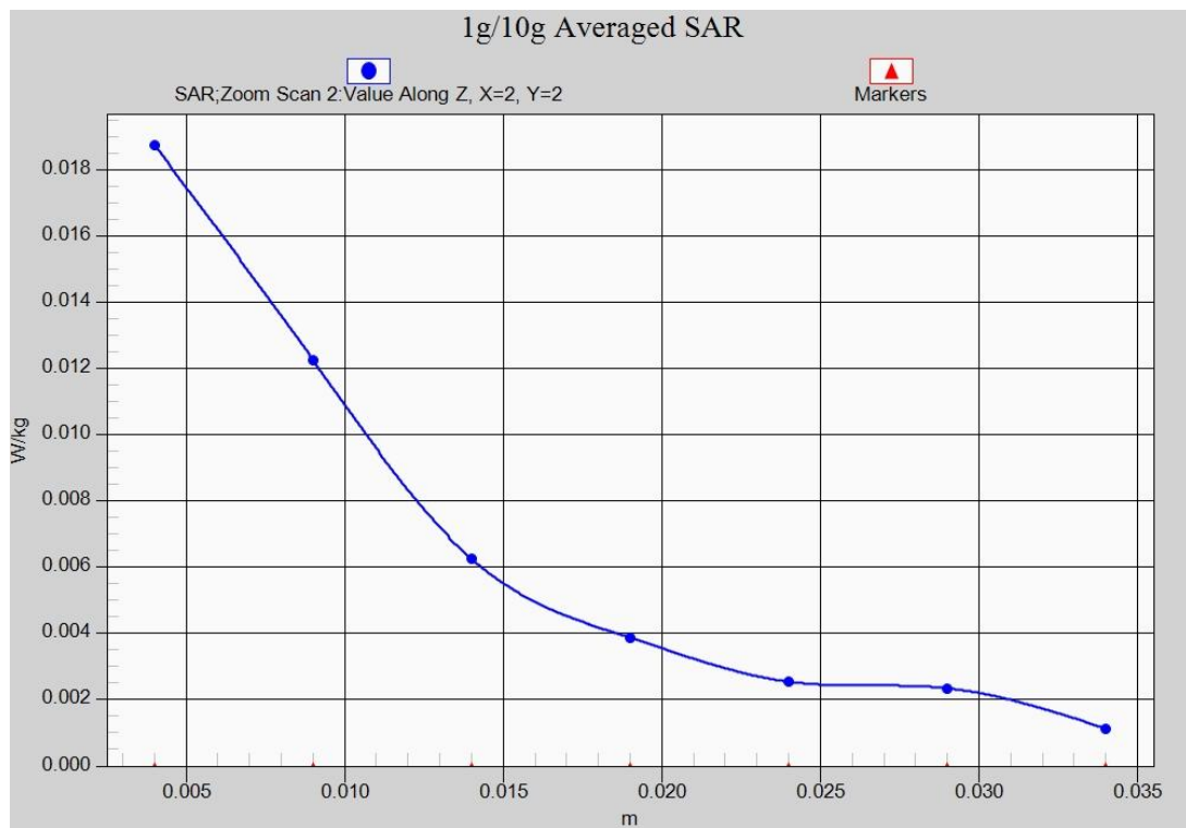
Fig. 10 -1 Z-Scan at power reference point (2450 MHz CH11)
