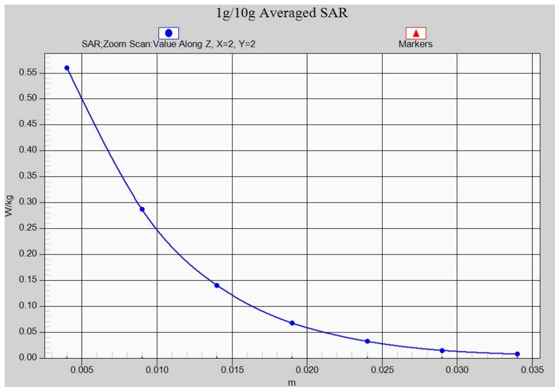
Fig. 9-1 Z-Scan at power reference point (2450 MHz CH11)
