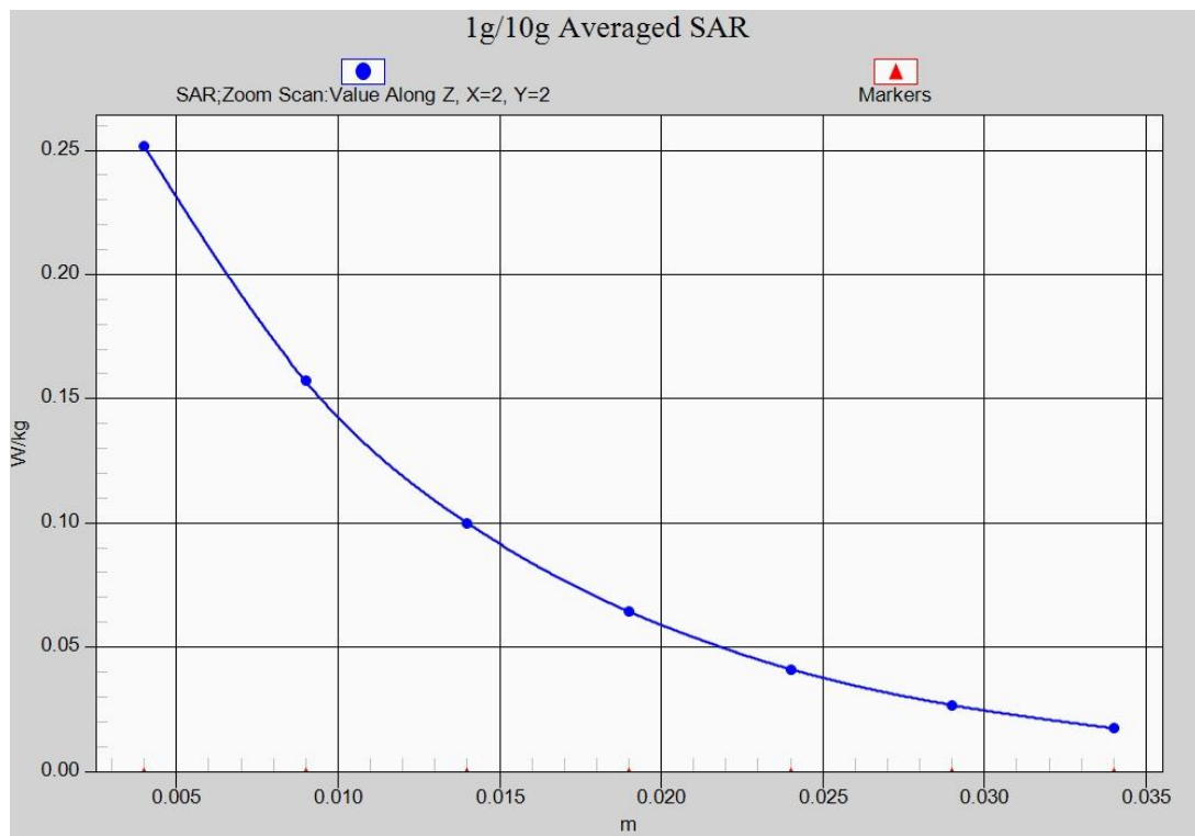
Fig. 7-1 Z-Scan at power reference point (WCDMA1900 CH9400)
