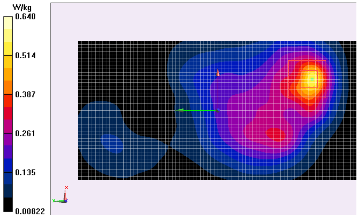
Fig.4 1900 MHz CH661
