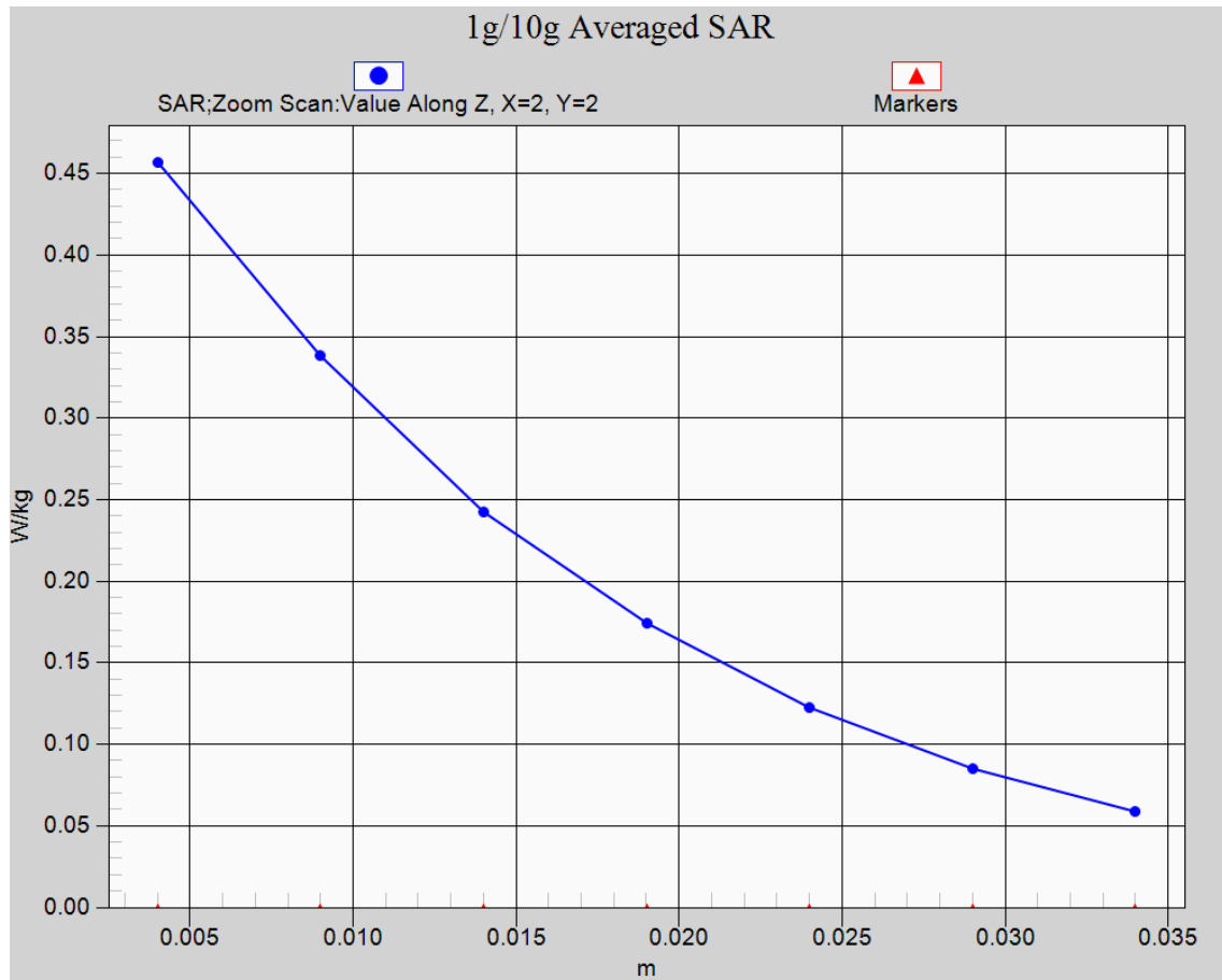
Fig. 8-1 Z-Scan at power reference point (WCDMA1900 CH9262)
