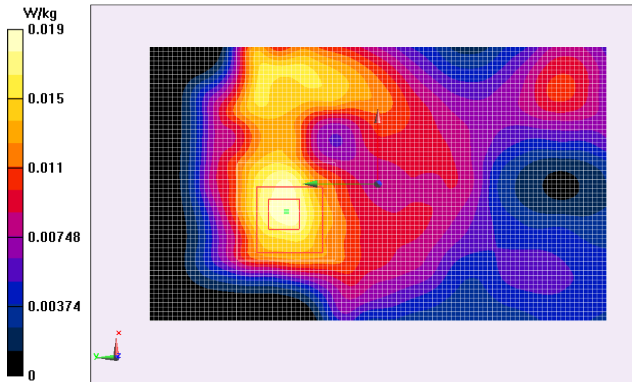
Fig.10 2450 MHz CH11
