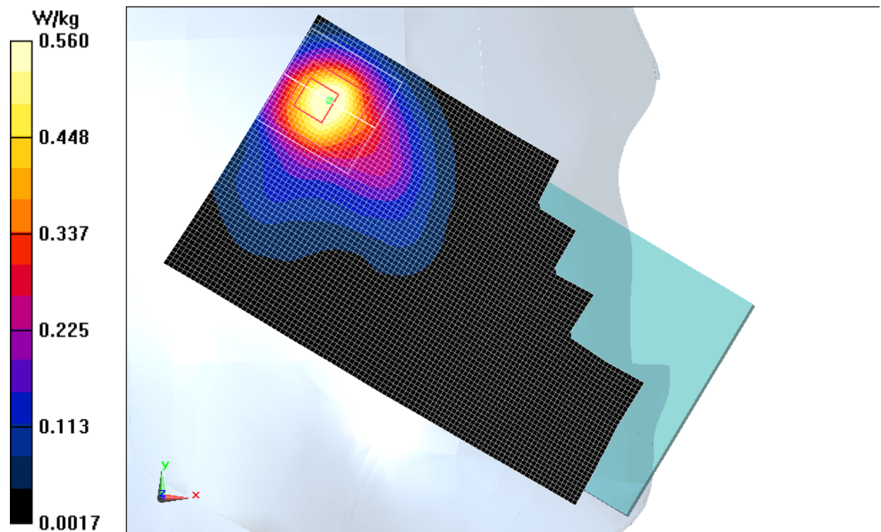
Fig.9 2450 MHz CH11
