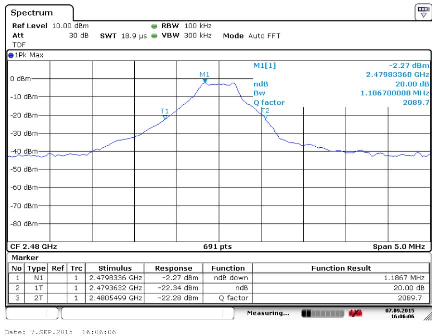
Fig. 74 Occupied 20dB Bandwidth (GFSK, Ch 78)
