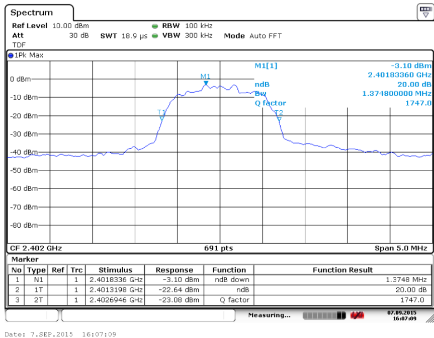
Fig. 78 Occupied 20dB Bandwidth (8DPSK, Ch 0)
