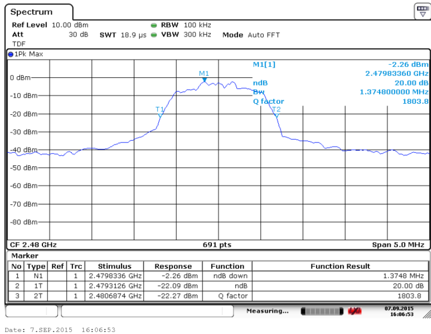
Fig. 77 Occupied 20dB Bandwidth ( \pi /4 DQPSK, Ch 78)
