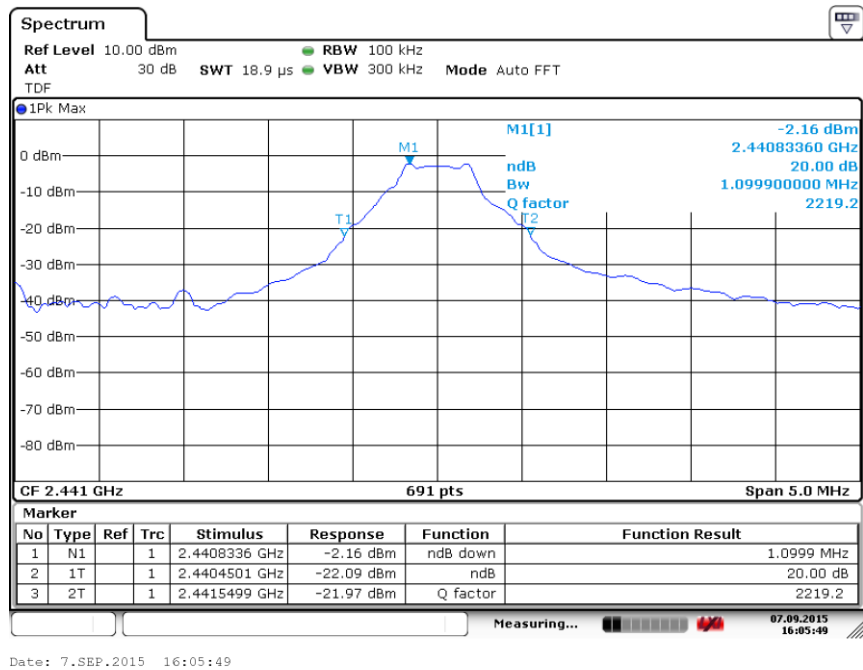
Fig. 73 Occupied 20dB Bandwidth (GFSK, Ch 39)
