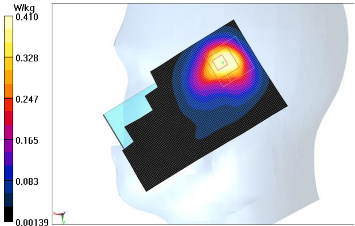
Fig.11 2450 MHz CH11
