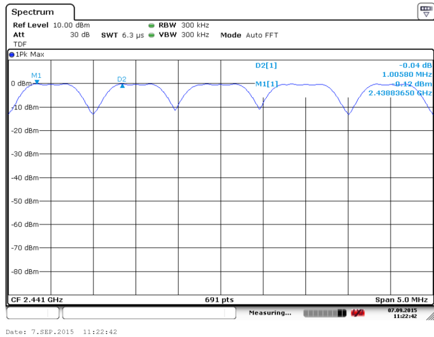
Fig. 93 Carrier Frequency Separation (GFSK, Ch39)
