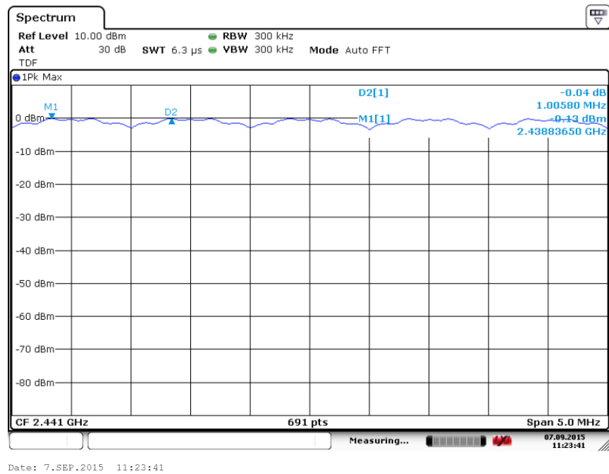
Fig. 94 Carrier Frequency Separation ( \pi/4 DQPSK, Ch39)
