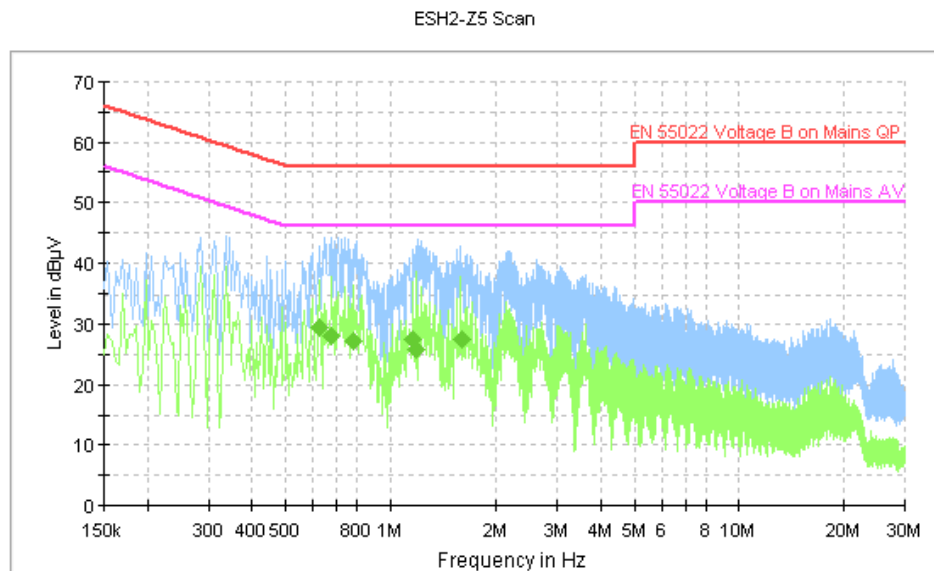
Fig. 99 AC Power line Conducted Emission (Traffic, AE1)
