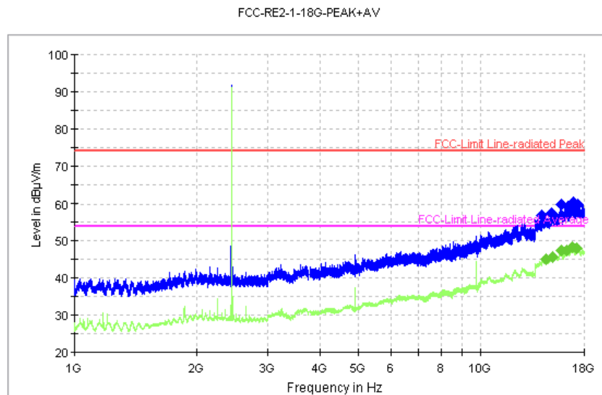
Fig. 53 Radiated Spurious Emission (GFSK, Ch39, 1 GHz ~18 GHz)
