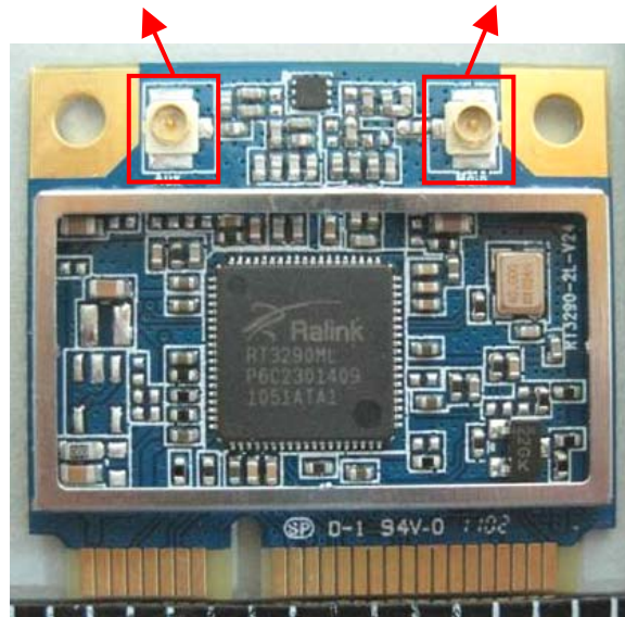
Connector 1: TX/RX (Main port)
