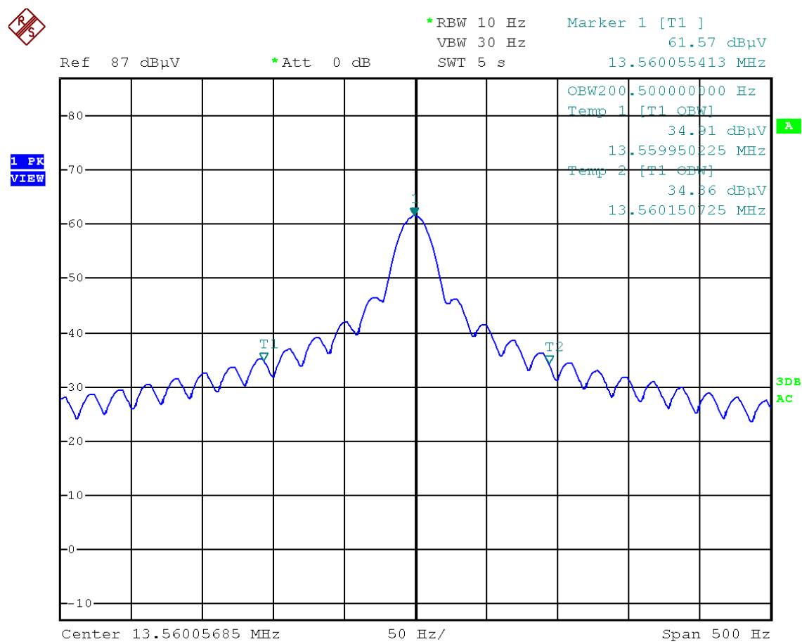
Figure 11: Chart of occupied bandwidth test
