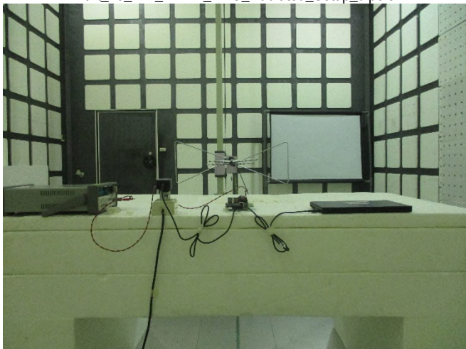
Part_15_247_WLAN_2.4G_Radiated_Setup_dipole
