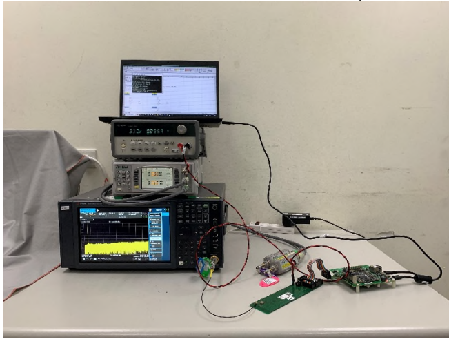
Part_15_247_WLAN_2.4G_Radiated_Setup_monopole
