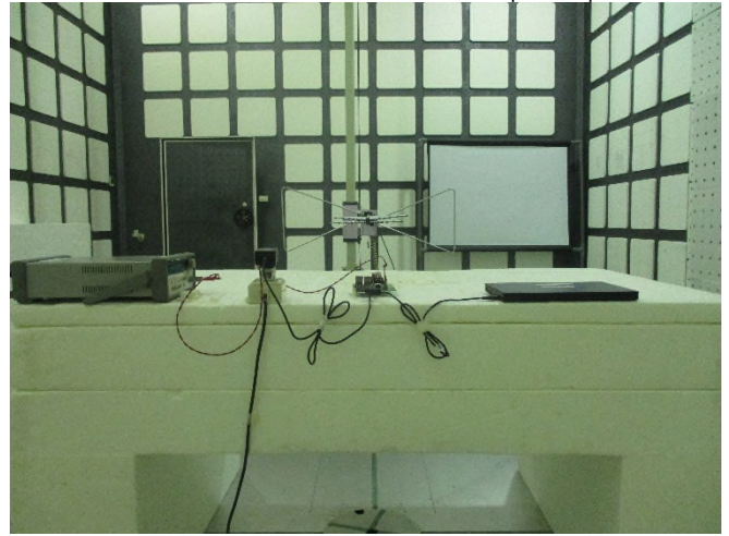
Part_15_247_WLAN_2.4G_Radiated_Setup_monopole
