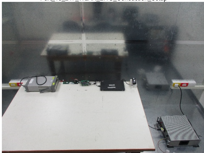
Part_15_247_WLAN_2.4G_Conduction_Setup
