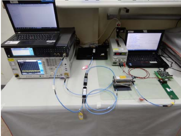
Part 15 407 WLAN 5G Normal DFS Setup
