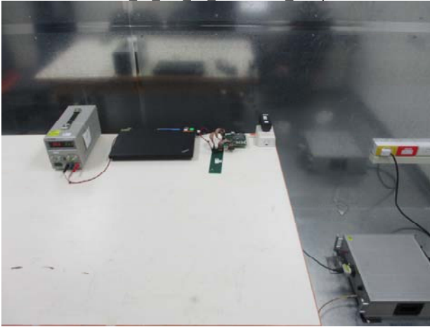
Part 15 247 LE Conduction Setup
