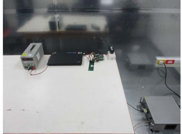
Part_15_247_BT_Conduction_Setup
