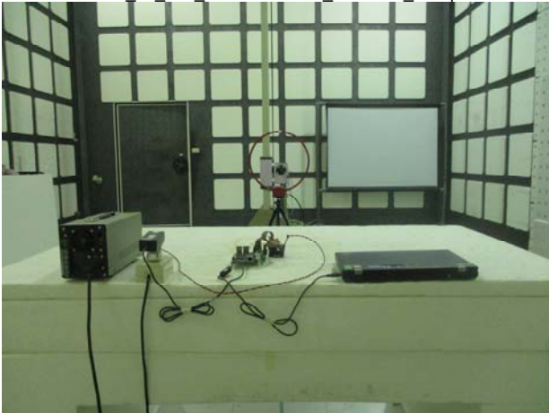
Part 15 247 IEEE 802.15.4 Radiated Setup
