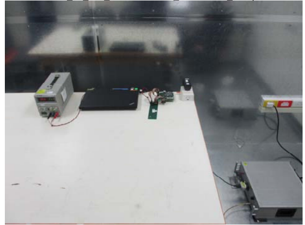
Part 15 247 IEEE 802.15.4 Conduction Setup
