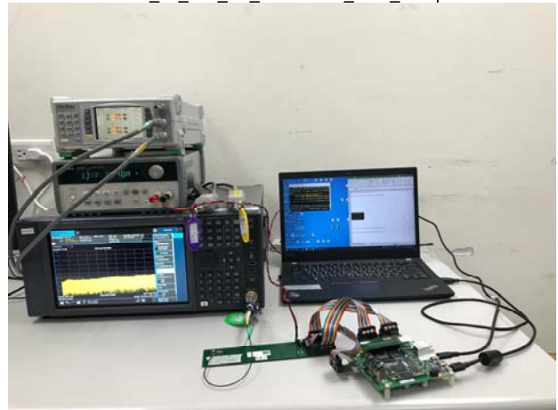
Part_15_247_BT_Conducted_Ant1_Setup
