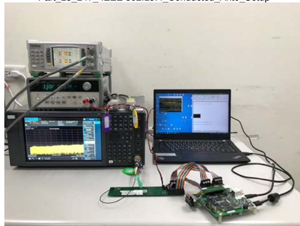
Part_15_247_IEEE 802.15.4_Conducted_Ant1_Setup
