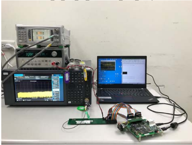
Part_15_247_LE_Conducted_Ant1_Setup
