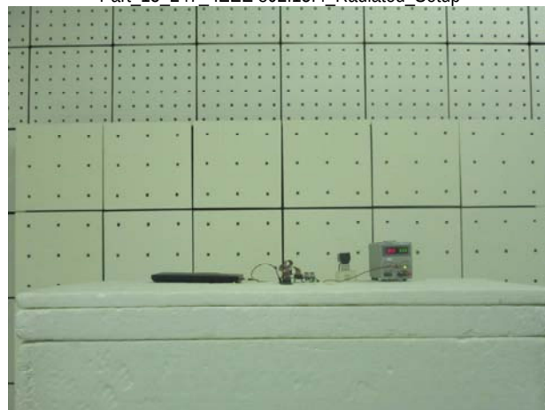
Part_15_247_IEEE 802.15.4_Radiated_Setup
