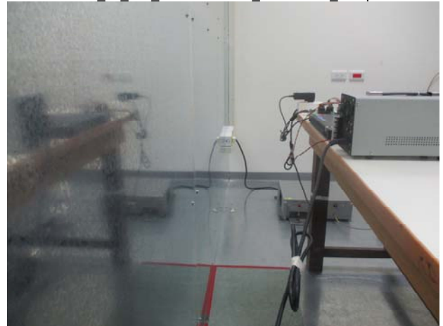
Part 15 407 WLAN 5G Conducted Setup
