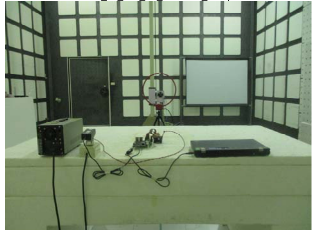
Part_15_247_LE_Radiated_Setup
