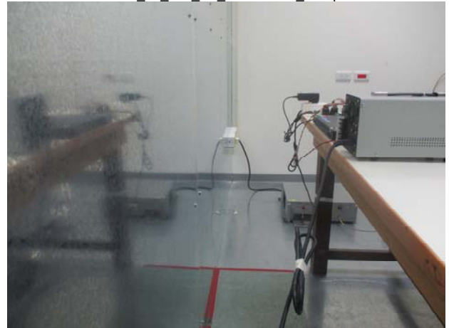
Part_15_247_BT_Conduction_Setup
