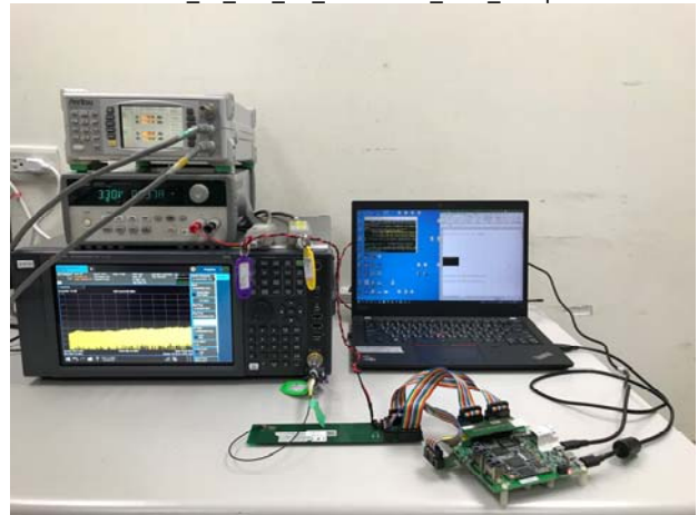
Part_15_247_BT_Conducted_Ant1_Setup
