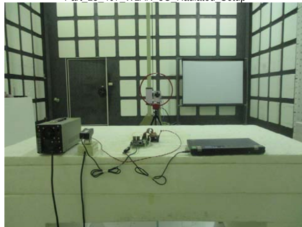
Part 15 407 WLAN 5G Conduction Setup
