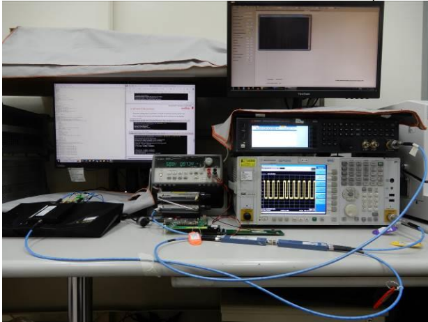
FCC_15_407&amp;RSS_247_WLAN_Normal_DFS_Setup
