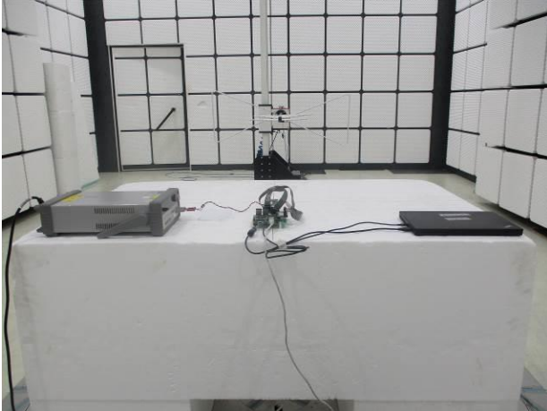
FCC_15_247&RSS_247_WLAN_Radiated_Internal antenna_Setup
