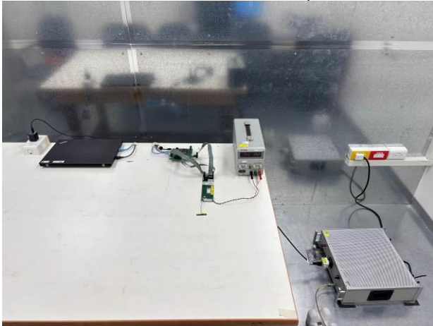
Co-location_Conduction_Setup
