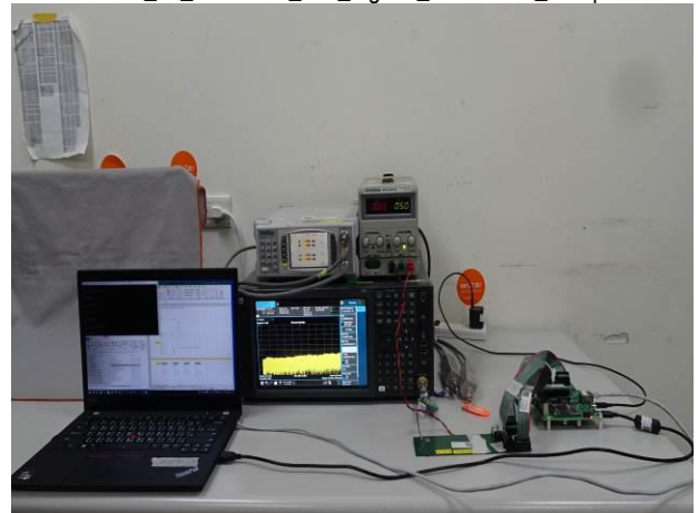
FCC_15_407&RSS_247_WLAN_Conducted_Setup
