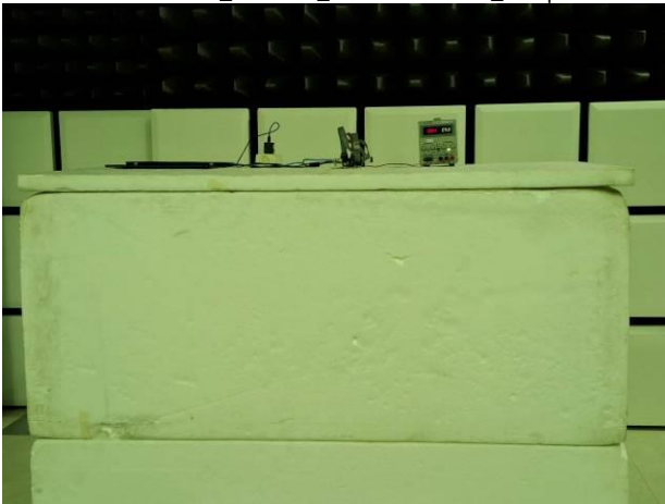
Co-location Radiated External antenna_Setup
