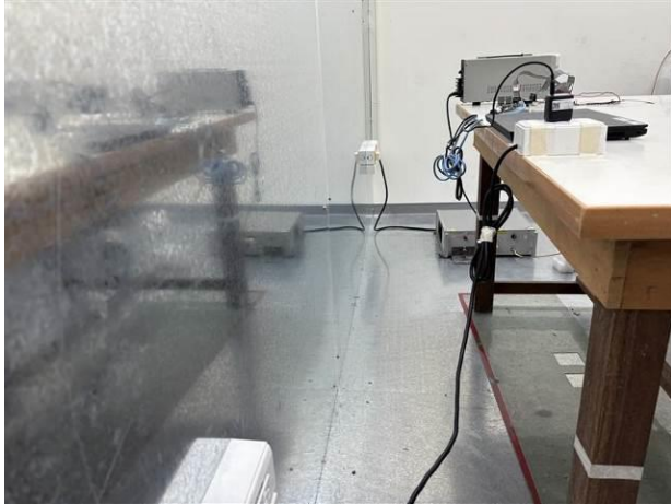
FCC_15_247&RSS_247_Zigbee_Conduction_Setup
