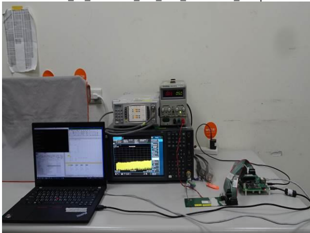
FCC_15_247&RSS_247_BLE_Conducted_Setup
