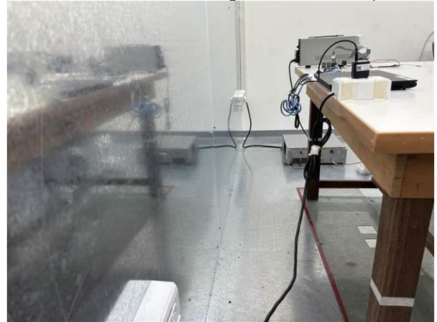
FCC_15_407&RSS_247_WLAN_Conduction_Setup
