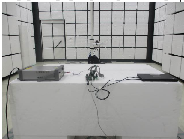
FCC 15 247&RSS 247 WLAN Radiated External antenna Setup
