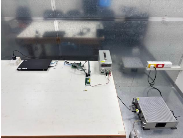
FCC_15_247&RSS_247_WLAN_Conduction_Setup
