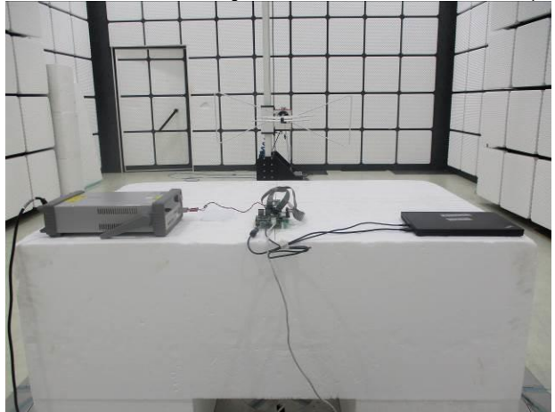
FCC 15 247&RSS 247 Zigbee Radiated Internal antenna Setup
