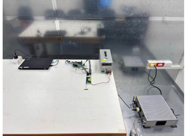
FCC_15_407&RSS_247_WLAN_Conduction_Setup
