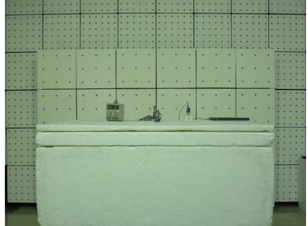
FCC_15_247&RSS_247_Zigbee_Radiated_External antenna_Setup
