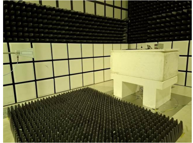
Co-location Radiated External antenna_Setup
