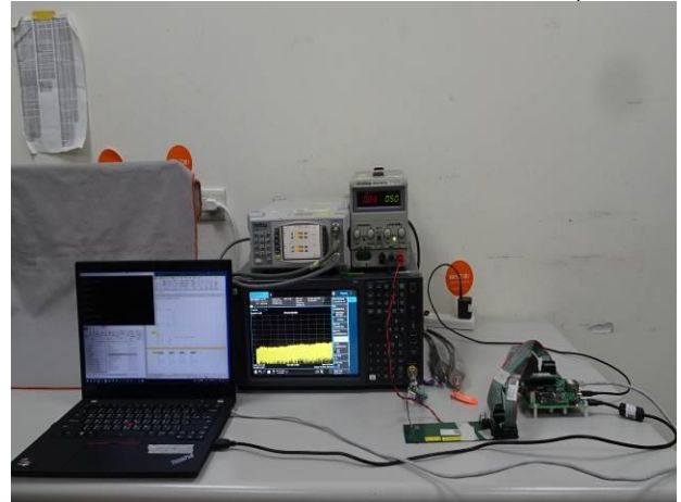
FCC_15_247&RSS_247_Zigbee_Conducted_Setup
