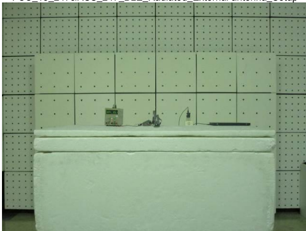
FCC_15_247&RSS_247_BLE_Radiated_External antenna_Setup
