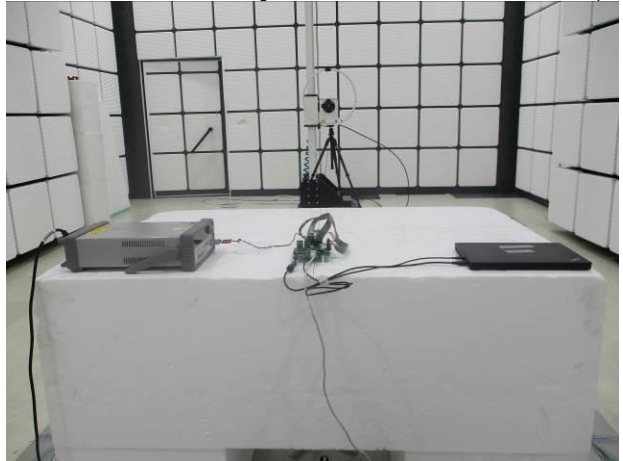
FCC 15 247&RSS 247 Zigbee Radiated Internal antenna Setup
