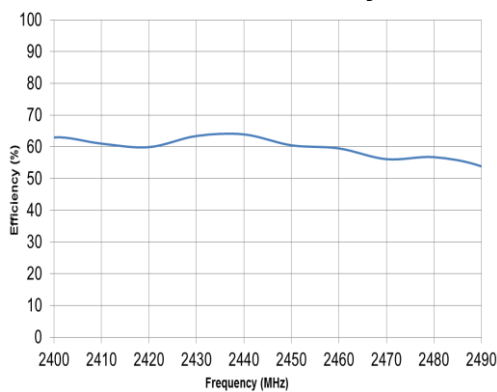
2.4 GHz Efficiency
