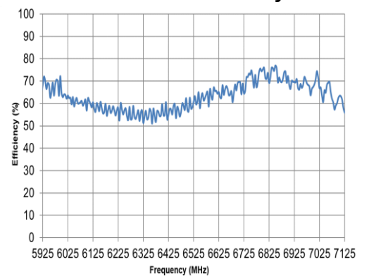
6 / 7 GHz Efficiency
