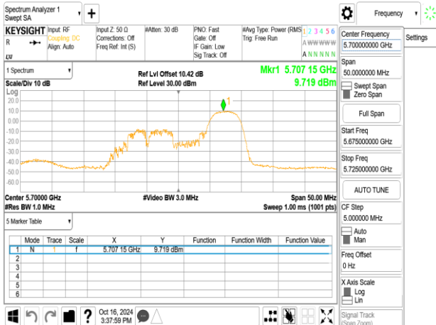
802.11ax_20MHz_Chain0_5700MHz_RU106_53
