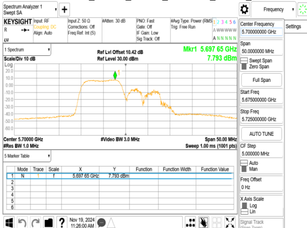
802.11ax_20MHz_Chain0_5700MHz_RU106_53
