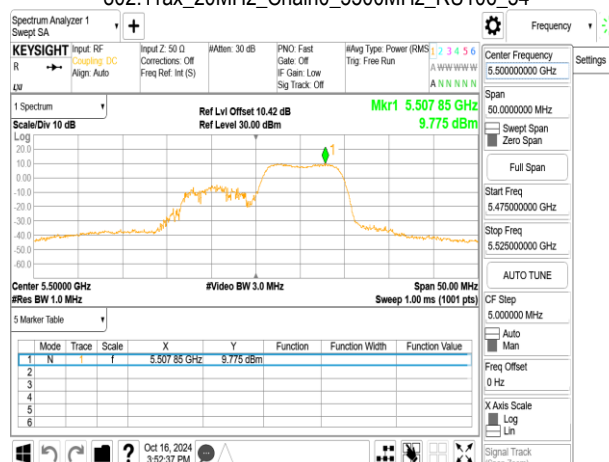
802.11ax_20MHz_Chain0_5500MHz_RU106_54
