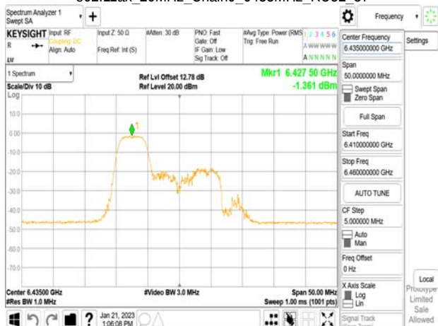
802.11ax_20MHz_Chain0_6435MHz_RU106_53
