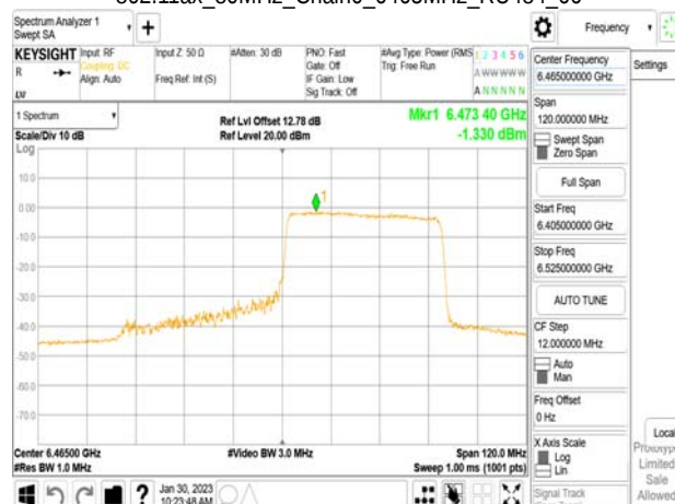
802.11ax_80MHz_Chain0_6465MHz_RU484_66
