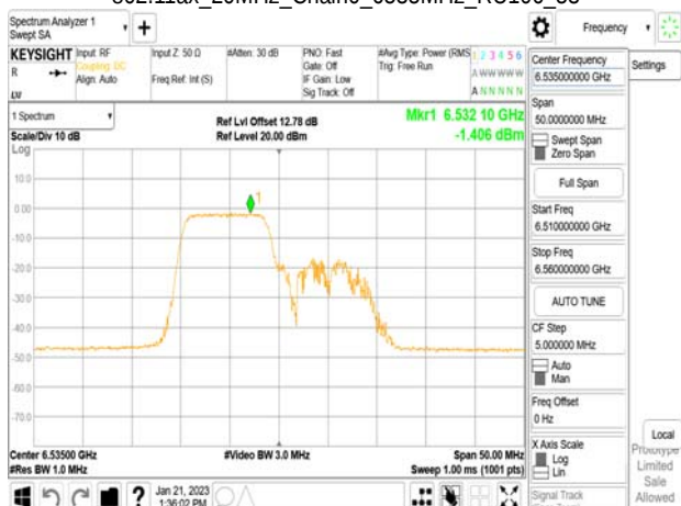
802.11ax_20MHz_Chain0_6535MHz_RU106_53
