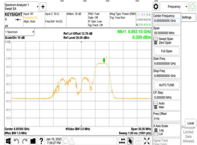
802.11ax_20MHz_Chain0_6855MHz_RU106_54
