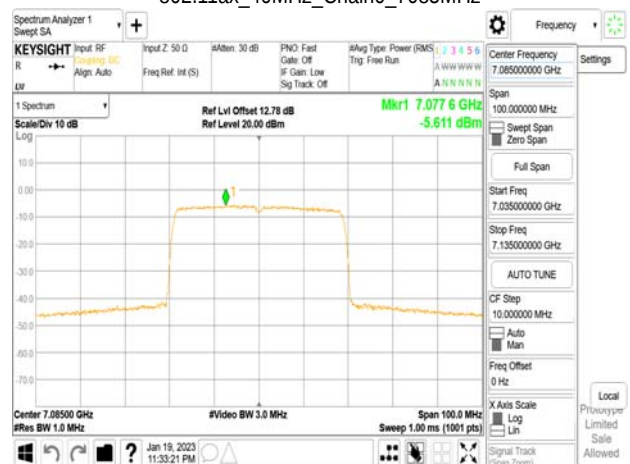
802.11ax_40MHz_Chain0_7085MHz
