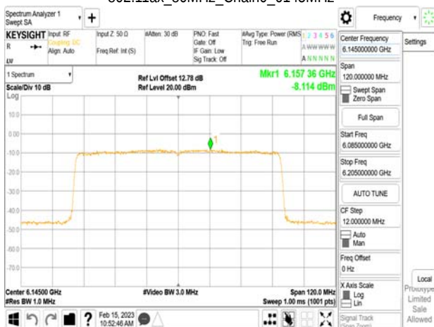
802.11ax_80MHz_Chain0_6145MHz
