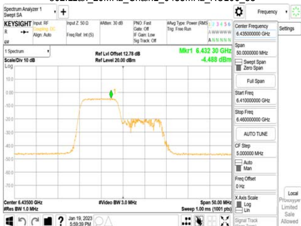
802.11ax_20MHz_Chain1_6435MHz_RU106_53
