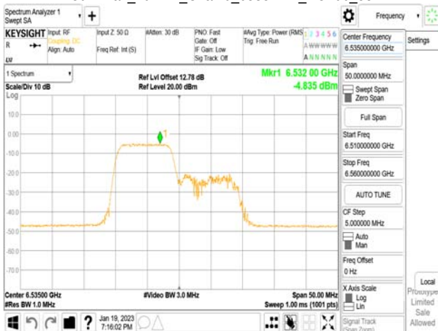
802.11ax_20MHz_Chain0_6535MHz_RU106_53
