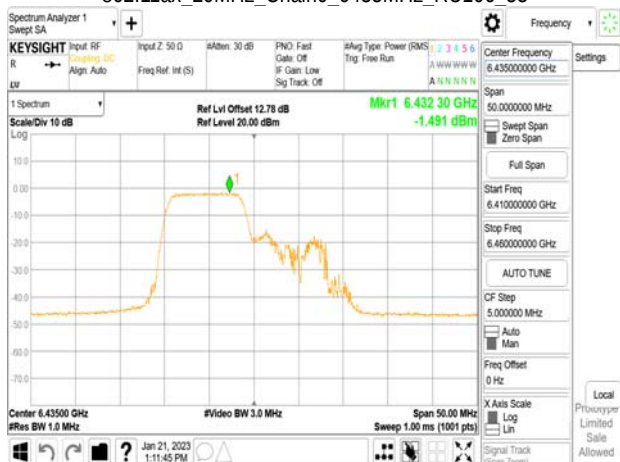
802.11ax_20MHz_Chain0_6435MHz_RU106_53
