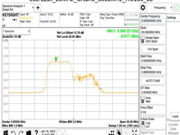
802.11ax_20MHz_Chain0_5955MHz_RU106_53
