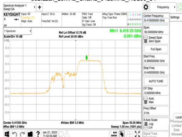
802.11ax_20MHz_Chain1_6415MHz_RU106_54
