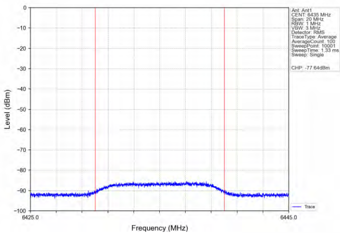
11AX20SISO-Ant 1-6435-Center-6435-Minimal
