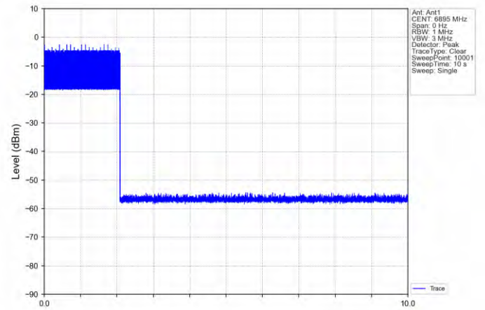
11AX20SISO-Ant 1-6895-Center-6895-OFF
