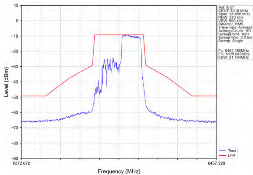
802.11ax(HE20)_HCH_6415MHz_RU106_Right_Ant1_NTNV
