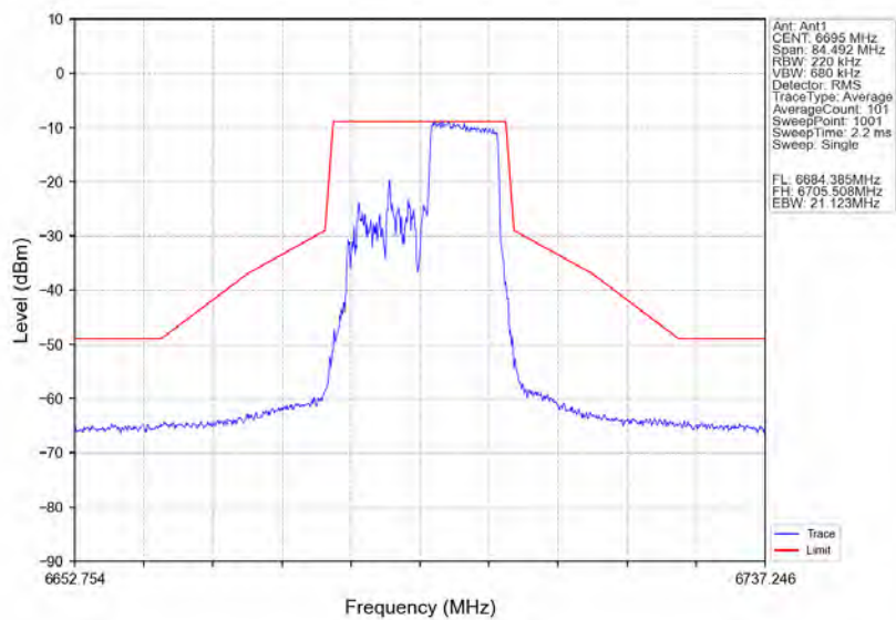
802.11ax(HE20)_MCH_6695MHz_RU106_Right_Ant1_NTNV
