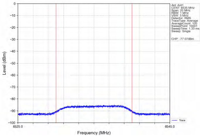
11AX20SISO-Ant 1-6535-Center-6535-Minimal
