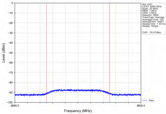
11AX20SISO-Ant 1-6895-Center-6895-Minimal
