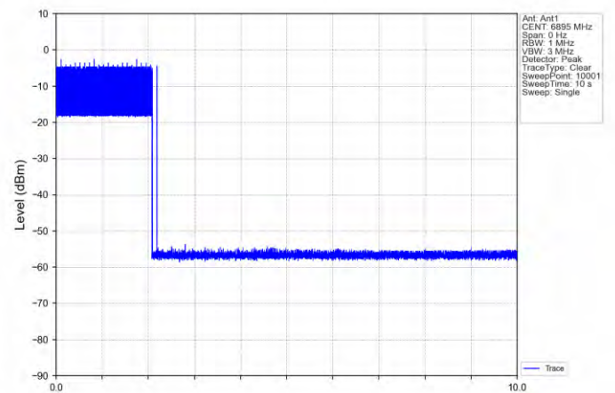
11AX20SISO-Ant 1-6895-Center-6895-Minimal
