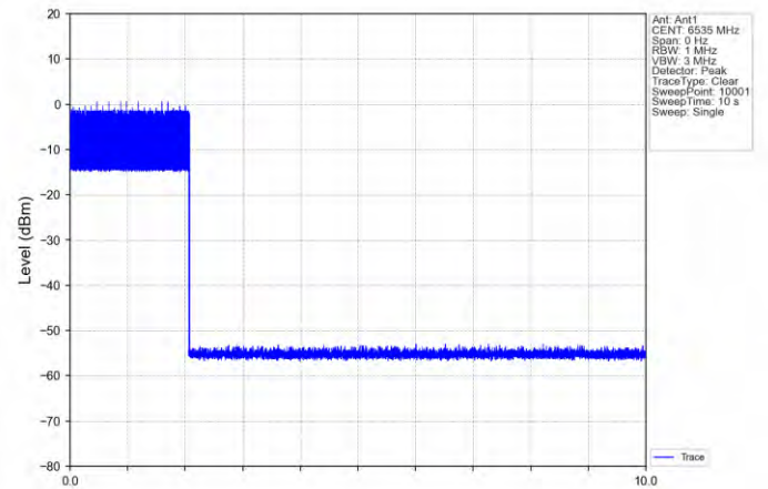
11AX20SISO-Ant 1-6535-Center-6535-OFF
