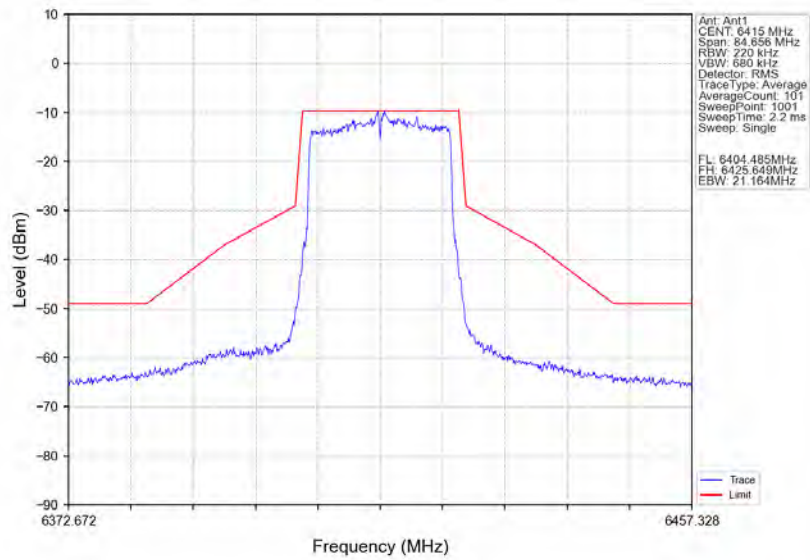
802.11ax(HE20)_HCH_6415MHz_RU242_Ant1_NTNV
