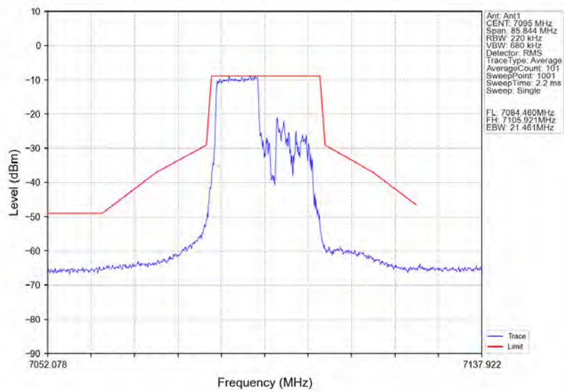
802.11ax(HE20)_HCH_7095MHz_RU106_Right_Ant1_NTNV
