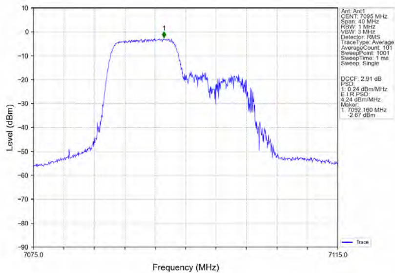
802.11ax(HE20)_HCH_7095MHz_RU106_Right_Ant1_NTNV
