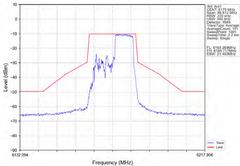
802.11ax(HE20)_MCH_6175MHz_RU106_Right_Ant1_NTNV
