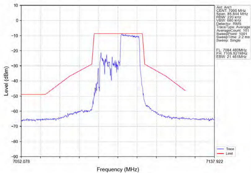
802.11ax(HE20)_HCH_7095MHz_RU106_Right_Ant1_NTNV
