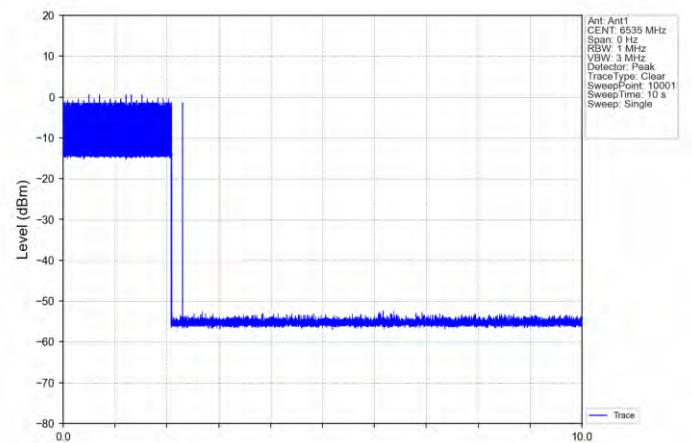
11AX20SISO-Ant 1-6535-Center-6535-Minimal
