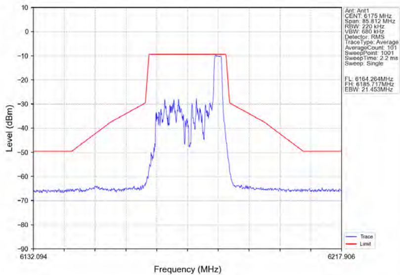
802.11ax(HE20)_MCH_6175MHz_RU26_Right_Ant1_NTNV
