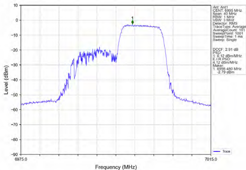
802.11ax(HE20)_MCH_6995MHz_RU106_Right_Ant1_NTNV
