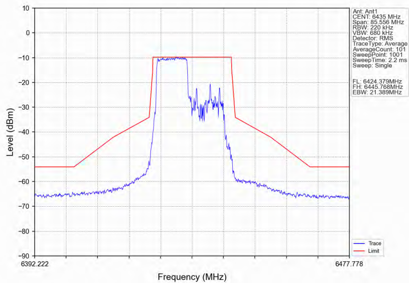
802.11ax(HE20)_LCH_6435MHz_RU106_Right_Ant1_NTNV
