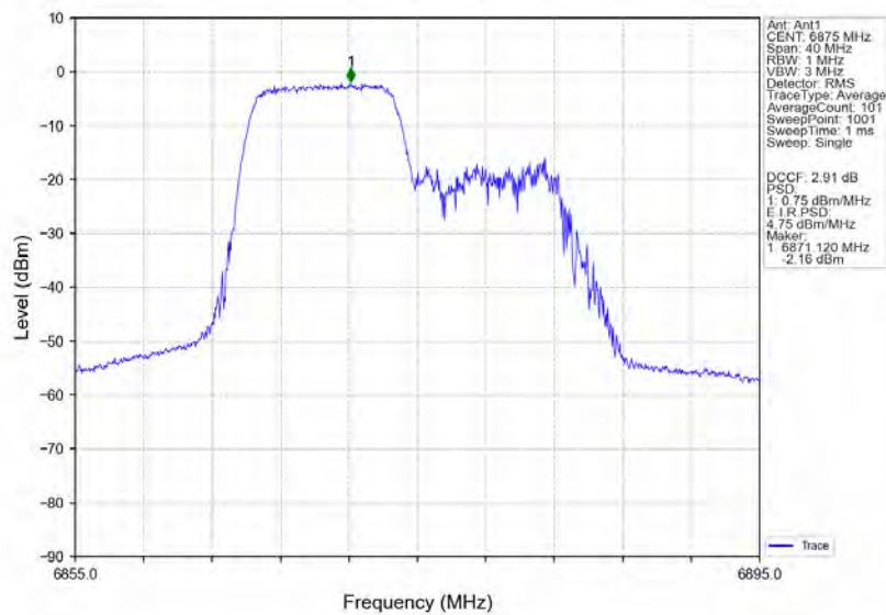
802.11ax(HE20)_HCH_6875MHz_RU106_Right_Ant1_NTNV
