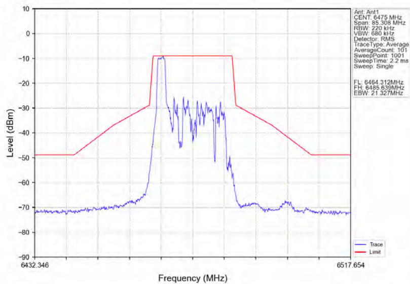
802.11ax(HE20)_MCH_6475MHz_RU26_Left_Ant1_NTNV
