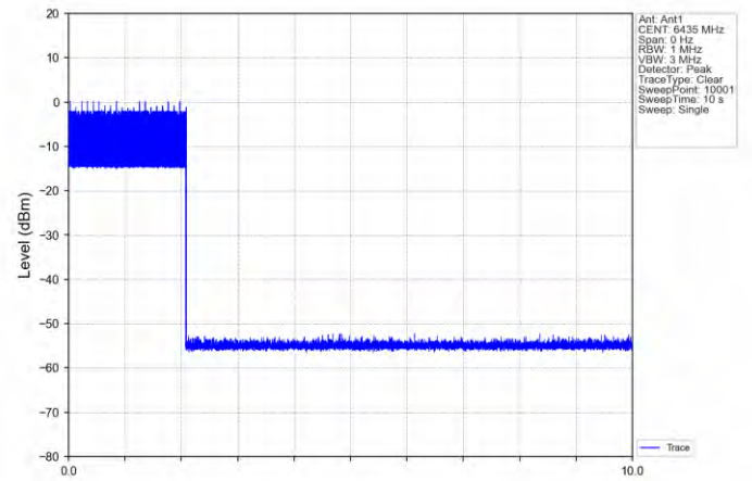
11AX20SISO-Ant 1-6435-Center-6435-OFF
