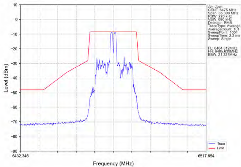
802.11ax(HE20)_MCH_6475MHz_RU26_Right_Ant1_NTNV
