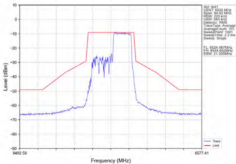
802.11ax(HE20)_LCH_6535MHz_RU106_Right_Ant1_NTNV
