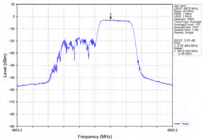
802.11ax(HE20)_HCH_6875MHz_RU106_Right_Ant1_NTNV
