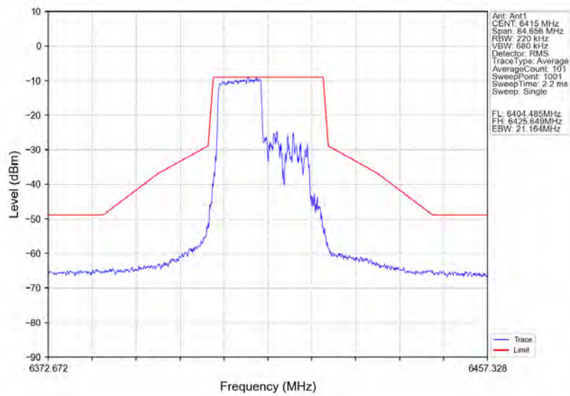
802.11ax(HE20)_HCH_6415MHz_RU106_Right_Ant1_NTNV
