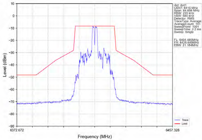
802.11ax(HE20)_HCH_6415MHz_RU26_Right_Ant1_NTNV
