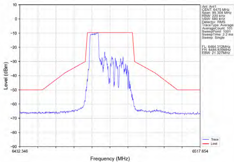
802.11ax(HE20)_MCH_6475MHz_RU52_Right_Ant1_NTNV
