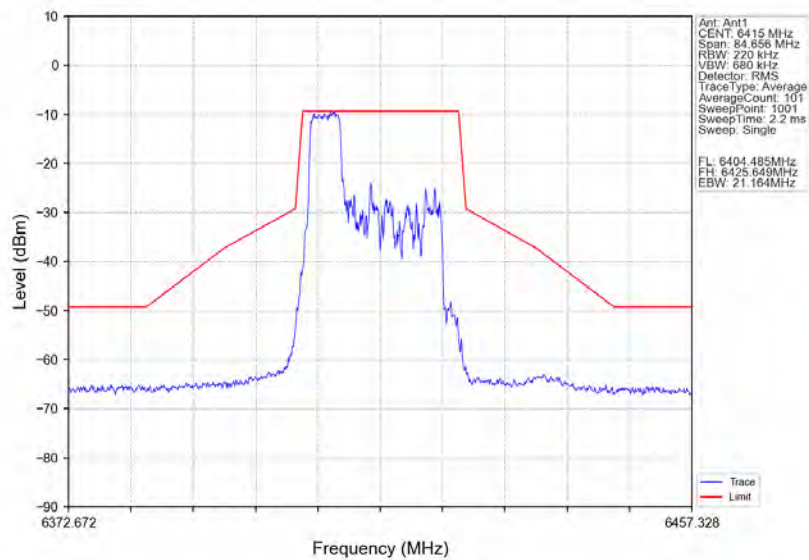
802.11ax(HE20) HCH_6415MHz_RU52_Right_Ant1_NTNV
