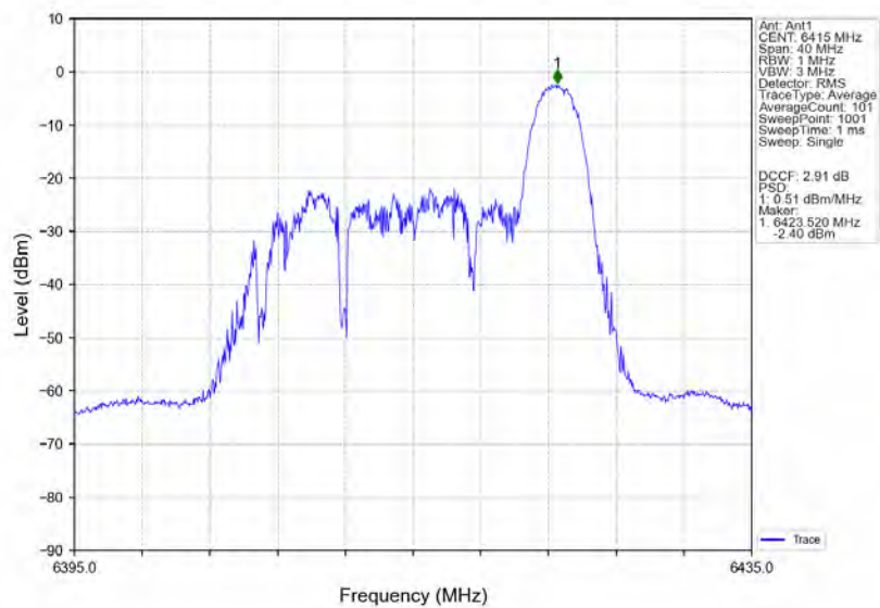
802.11ax(HE20) HCH_6415MHz_RU26_Right_Ant1_NTNV
