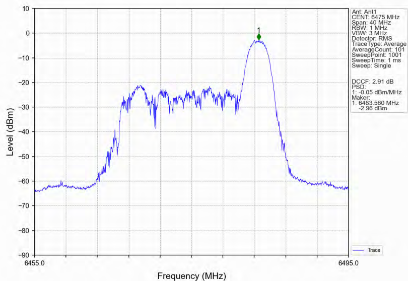
802.11ax(HE20)_MCH_6475MHz_RU26_Right_Ant1_NTNV
