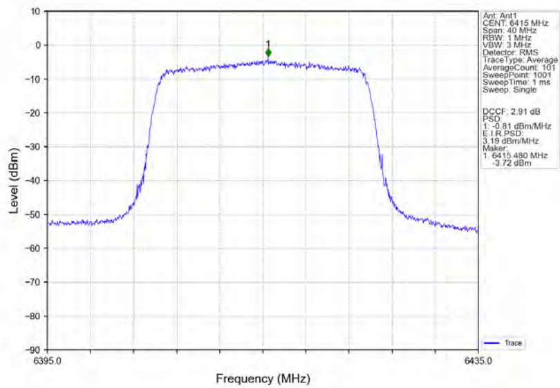
802.11ax(HE20)_HCH_6415MHz_RU242_Ant1_NTNV
