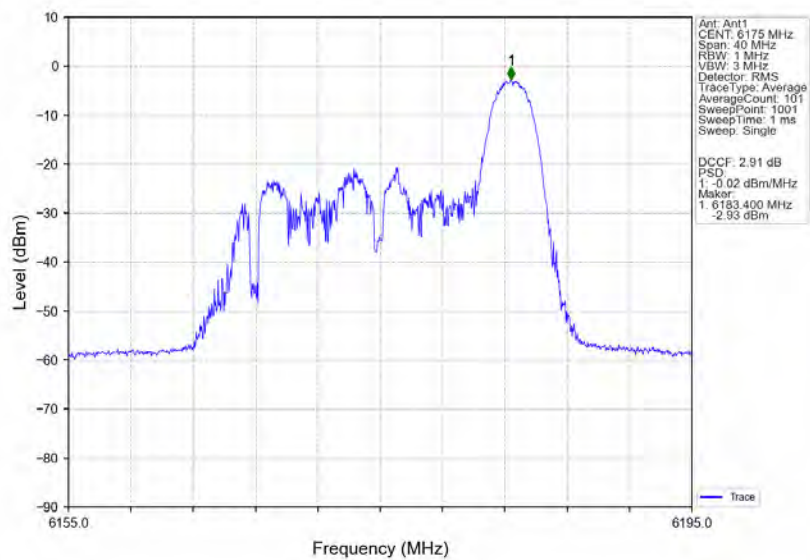
802.11ax(HE20)_MCH_6175MHz_RU26_Right_Ant1_NTNV
