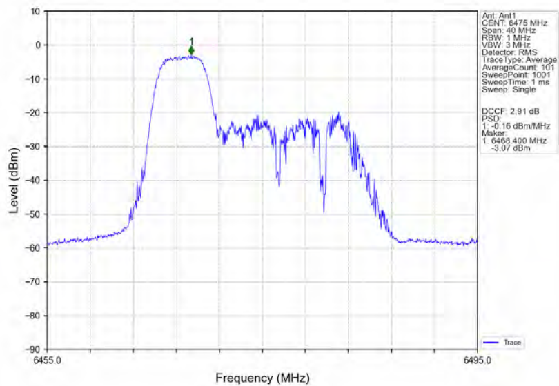
802.11ax(HE20)_MCH_6475MHz_RU52_Right_Ant1_NTNV
