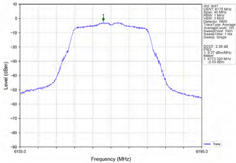
802.11a_MCH_6175MHz_Ant1_NTNV
