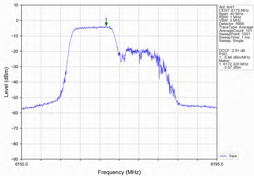
802.11ax(HE20)_MCH_6175MHz_RU106_Right_Ant1_NTNV
