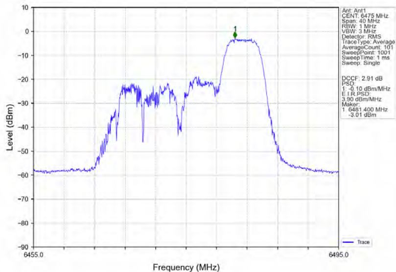
802.11ax(HE20)_MCH_6475MHz_RU52_Right_Ant1_NTNV
