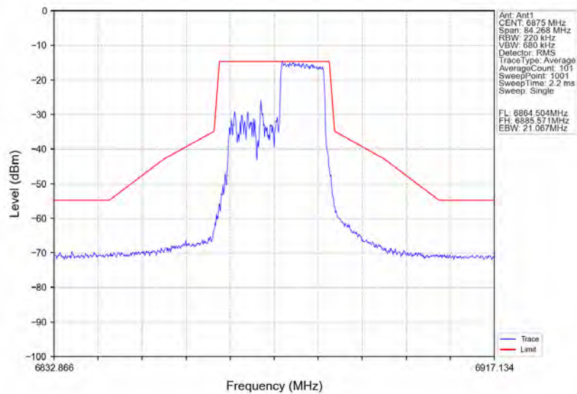
802.11ax(HE20)_HCH_6875MHz_RU106_Right_Ant1_NTNV
