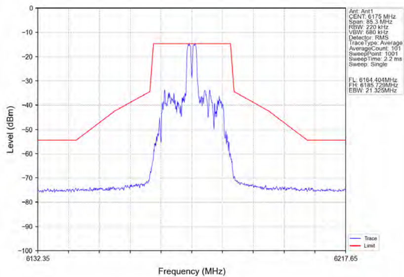
802.11ax(HE20)_MCH_6175MHz_RU26_Right_Ant1_NTNV
