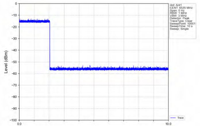
11AX20SISO-Ant 1-6535-Center-6535-OFF
