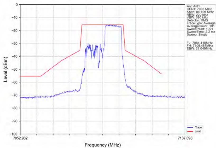
802.11ax(HE20)_HCH_7095MHz_RU106_Right_Ant1_NTNV
