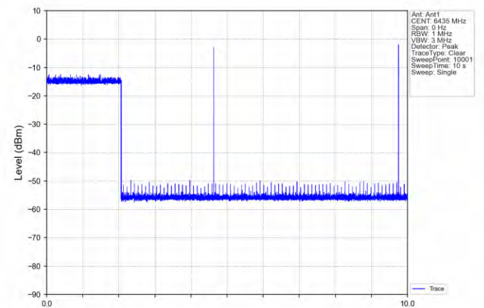
11AX20SISO-Ant 1-6435-Center-6435-Minimal
