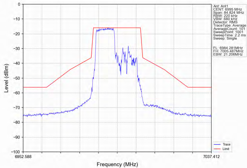
802.11ax(HE20)_MCH_6995MHz_RU106_Right_Ant1_NTNV
