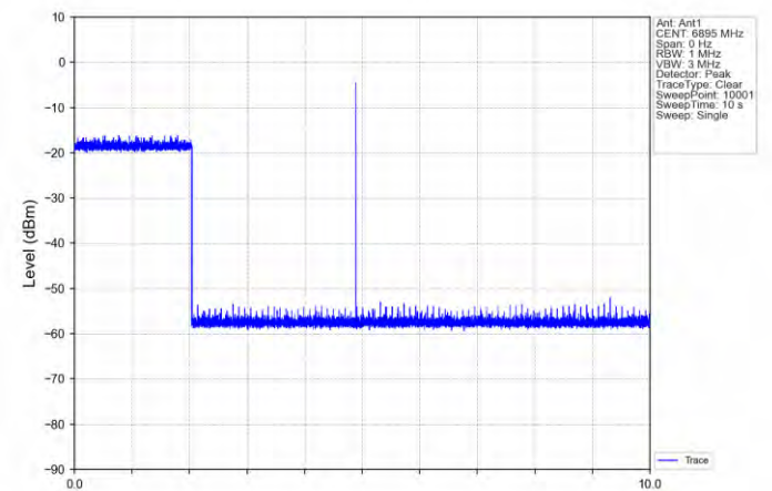
11AX20SISO-Ant 1-6895-Center-6895-Minimal
