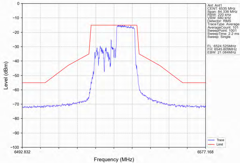
802.11ax(HE20)_LCH_6535MHz_RU106_Right_Ant1_NTNV
