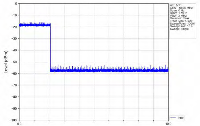
11AX20SISO-Ant 1-6895-Center-6895-OFF
