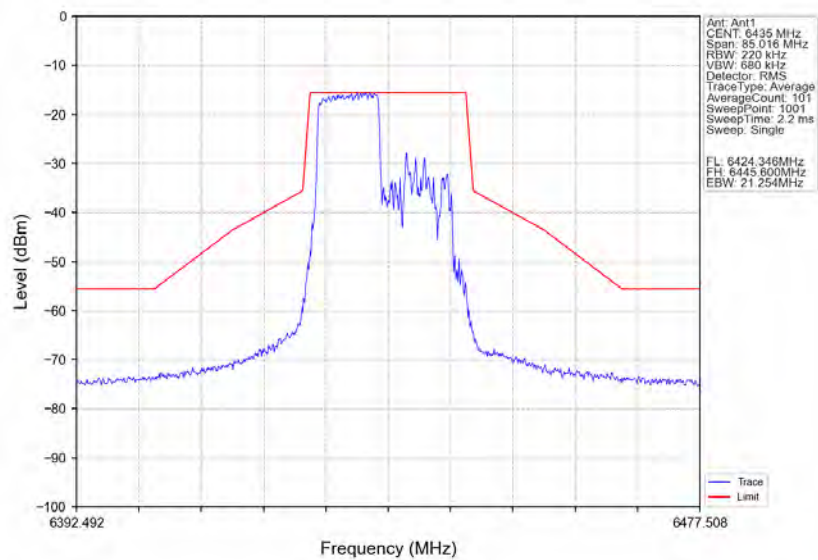
802.11ax(HE20)_LCH_6435MHz_RU106_Right_Ant1_NTNV
