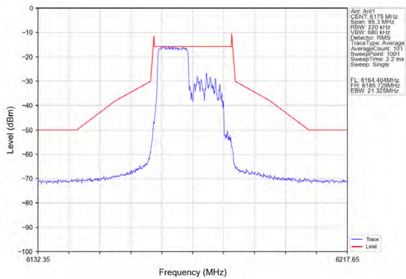
802.11ax(HE20)_MCH_6175MHz_RU106_Right_Ant1_NTNV
