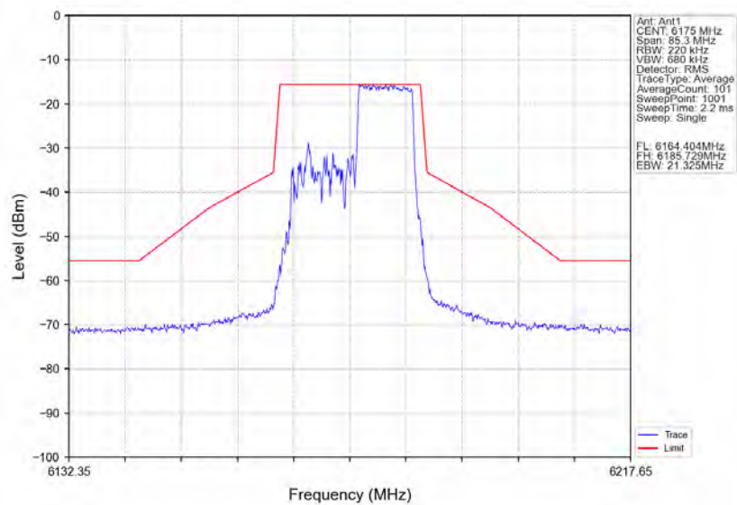
802.11ax(HE20)_MCH_6175MHz_RU106_Right_Ant1_NTNV
