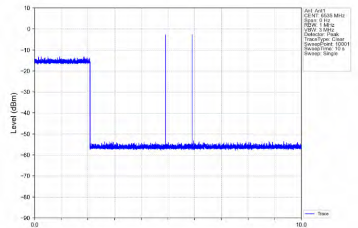
11AX20SISO-Ant 1-6535-Center-6535-Minimal
