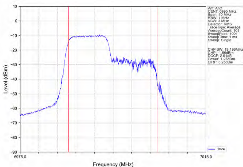
802.11ax(HE20)_MCH_6995MHz_RU106_Right_Ant1_NTNV
