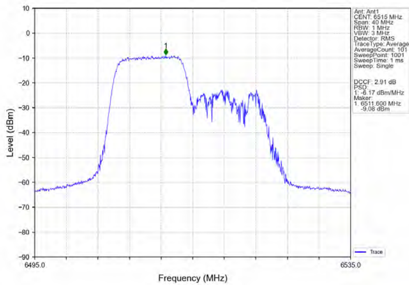
802.11ax(HE20)_HCH_6515MHz_RU106_Right_Ant1_NTNV
