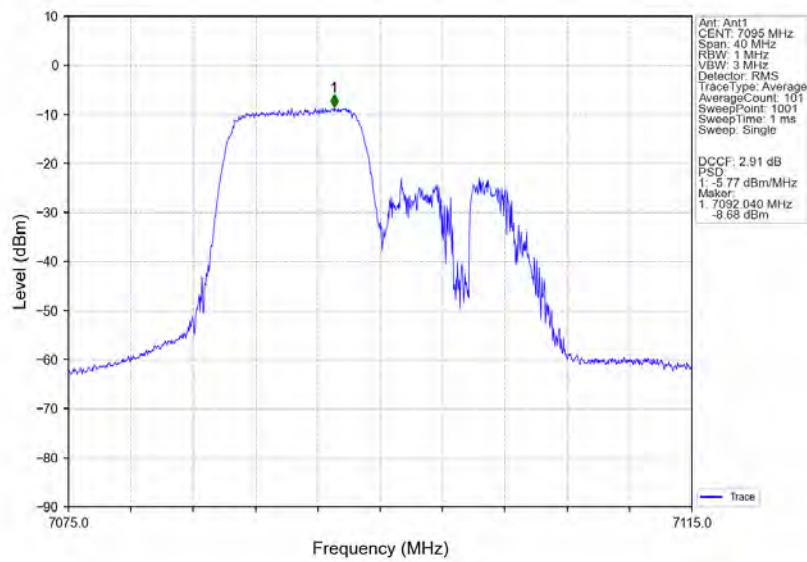
802.11ax(HE20)_HCH_7095MHz_RU106_Right_Ant1_NTNV
