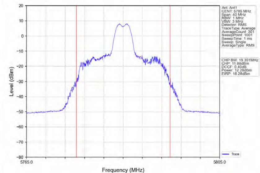
802.11ax(HE20)_MCH_5785MHz_RU26_Mid_Ant1_NTNV
