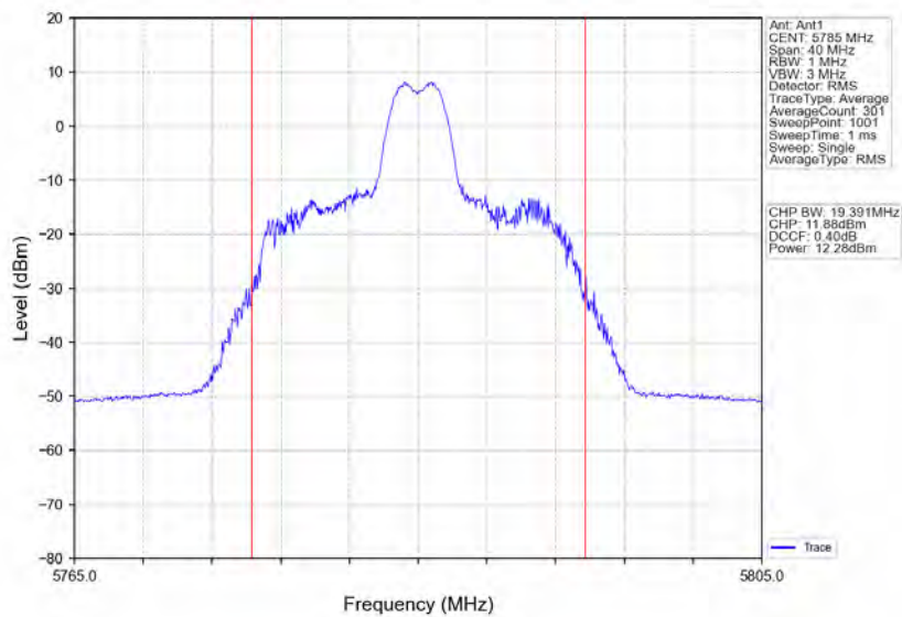
802.11ax(HE20)_MCH_5785MHz_RU26_Mid_Ant1_NTNV
