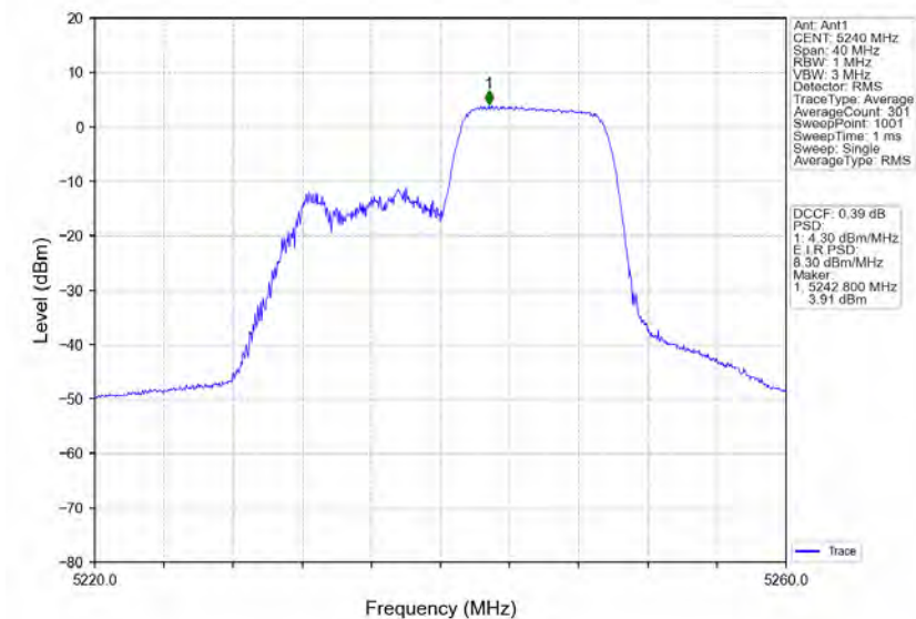
802.11ax(HE20)_HCH_5240MHz_RU106_Right_Ant1_NTNV
