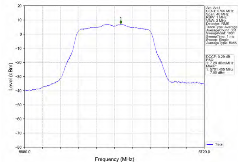
802.11a_HCH_5700MHz_Ant1_NTNV
