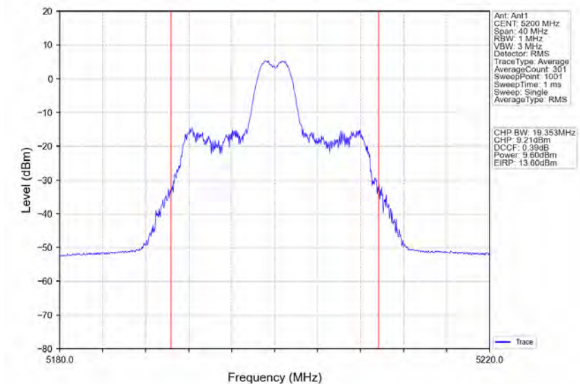
802.11ax(HE20)_MCH_5200MHz_RU26_Mid_Ant1_NTNV
