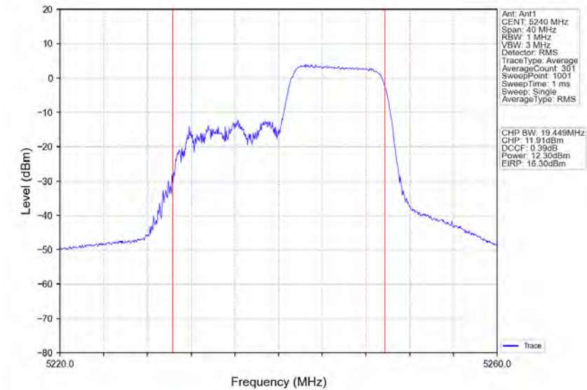
802.11ax(HE20)_HCH_5240MHz_RU106_Right_Ant1_NTNV
