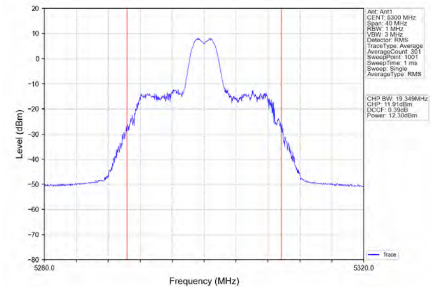
802.11ax(HE20)_MCH_5300MHz_RU26_Mid_Ant1_NTNV
