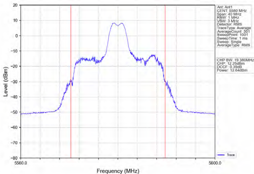
802.11ax(HE20)_MCH_5580MHz_RU26_Mid_Ant1_NTNV
