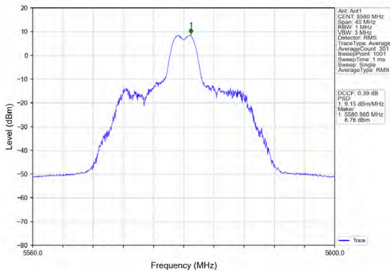
802.11ax(HE20)_MCH_5580MHz_RU26_Mid_Ant1_NTNV
