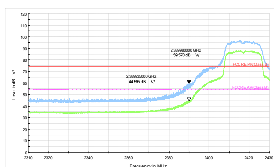
802.11n HT20-Channel 2 Peak+ Average
