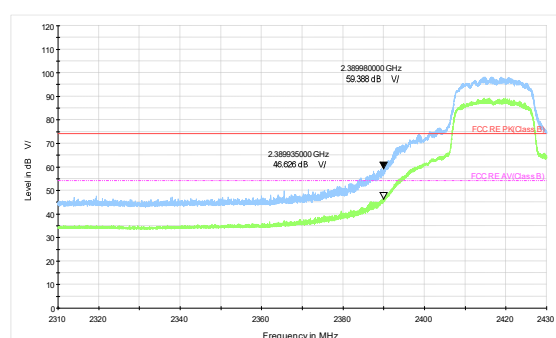
802.11ax HE20-Channel 2 Peak+ Average
