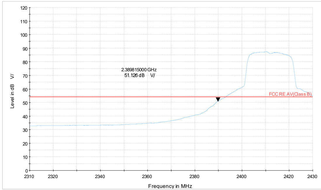
2.4G WIFI_ax20 CH1_2.31-2.43GHz_TP16.5_Y_242TONE_INDEX61_AV
