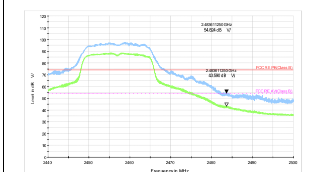
802.11g-Channel 10 Peak+ Average
