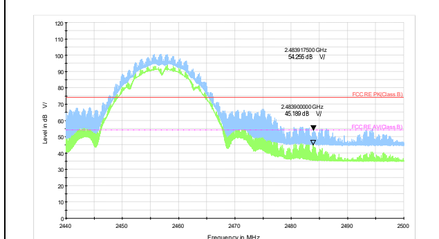
802.11b-Channel 10 Peak+ Average
