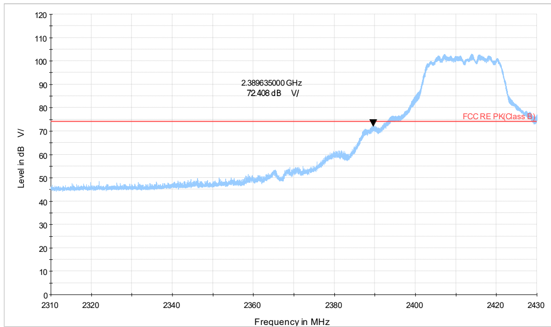
2.4G WIFI_ax20 CH1_2.31-2.43GHz_TP16.5_Y_242TONE_INDEX61_PK
