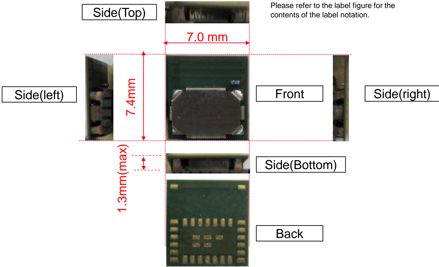
Surface mount type : 7.4 x 7.0 mm (Typical), H = 1.3 mm (Max)
