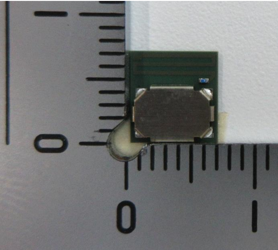
Module(Front)
