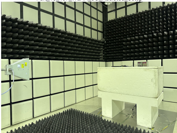
Part_15_407_WLAN_5G_Radiated_Setup
