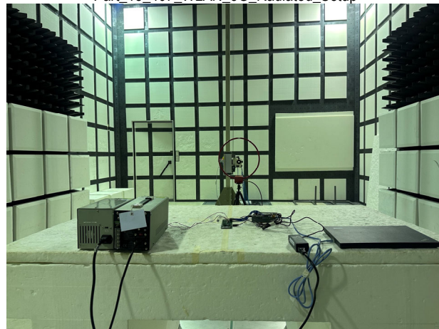
Part_15_407_WLAN_5G_Conducted_Setup
