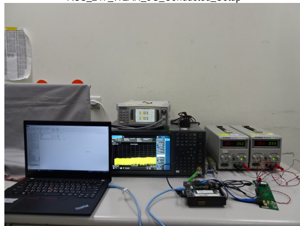
RSS_247_WLAN_5G_Conducted_Setup
