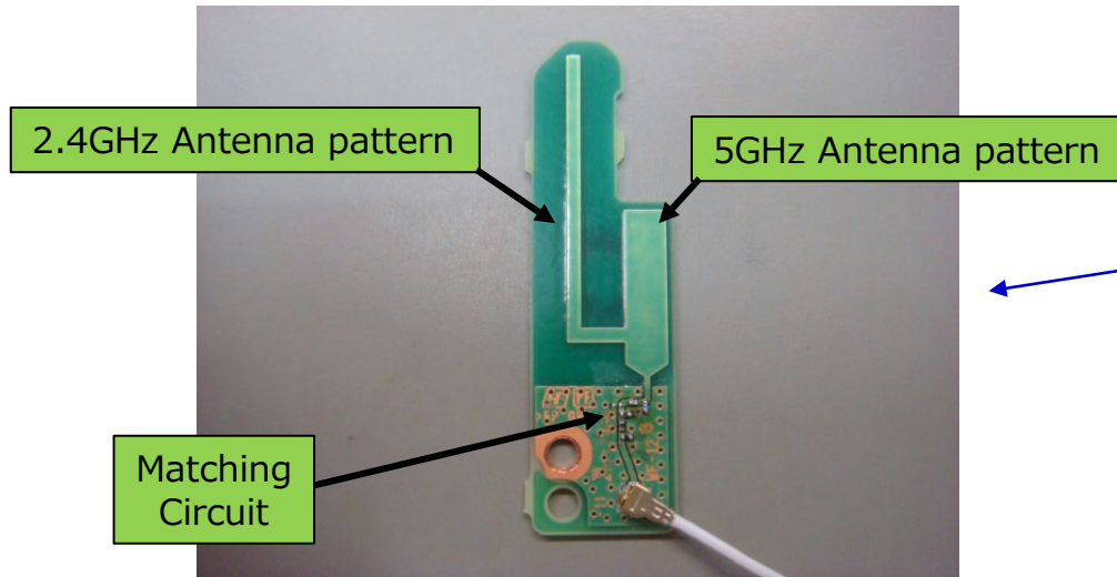
Dual Monopole Antenna "WF-12"
