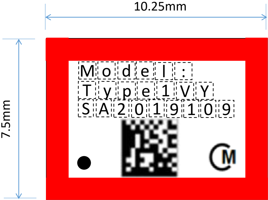
The red part is the print design prohibited area
