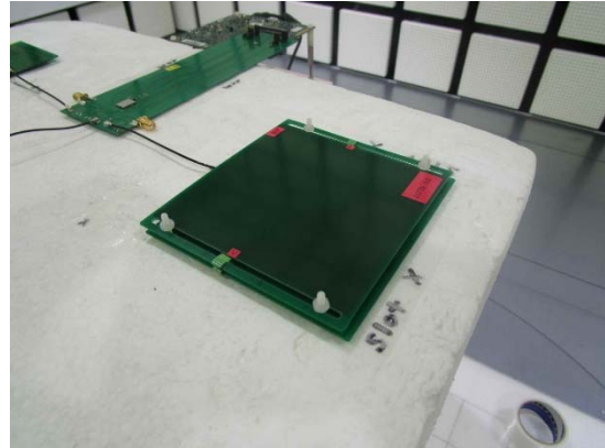
Slot Antenna X-axis
