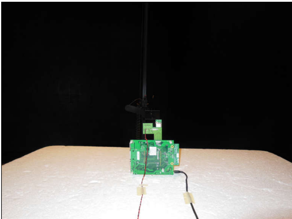
Figure 12: WiFi – YPOS
