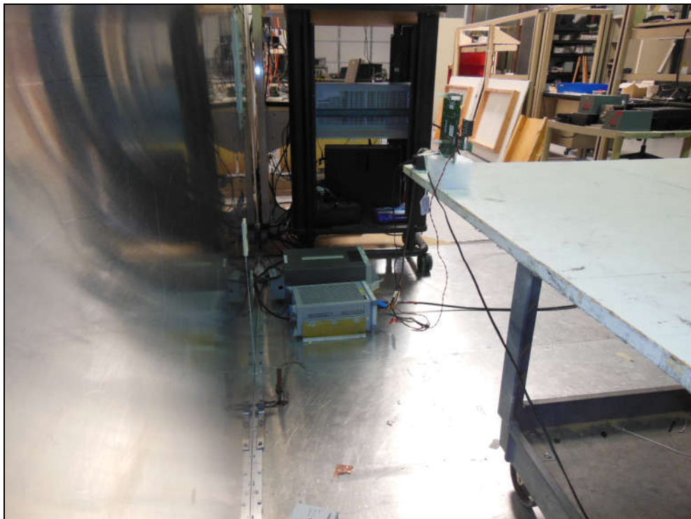
Figure 16: Conducted Emissions
