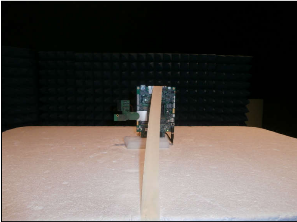
Figure 9: WiFi – XPOS
