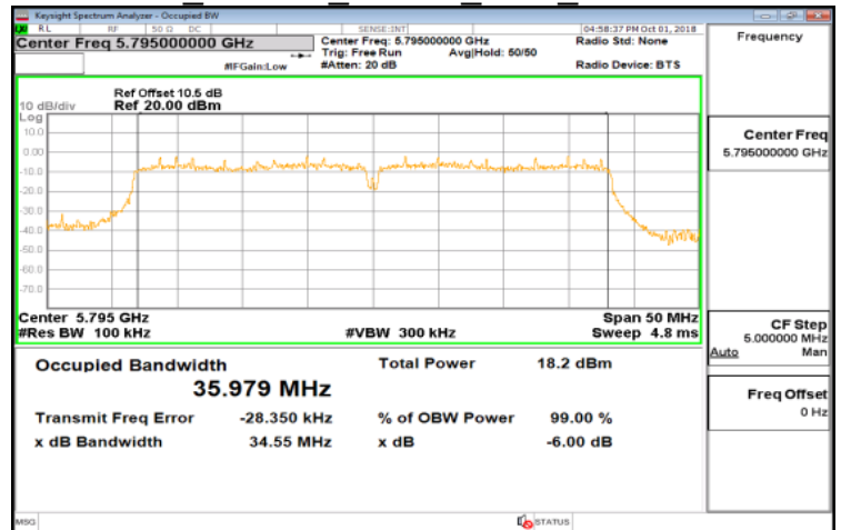
FCC 802.11n 40MHz Main 5795MHz
