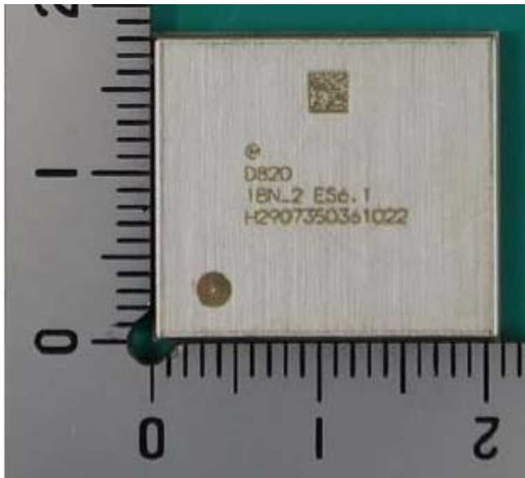
Back View of EUT
