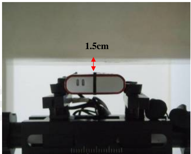
Fig.9 Body worn- EUT back to flat phantom with headset and distance between flat phantom and mobile phone is 1.5 cm
