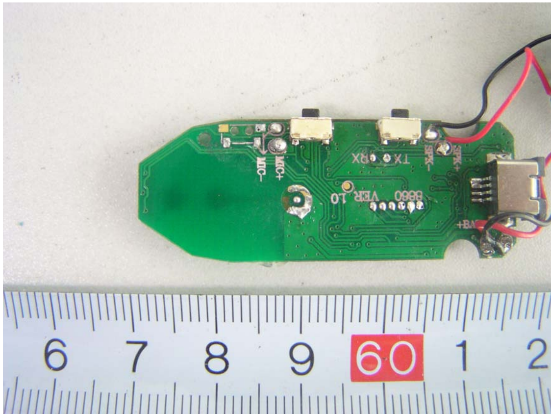
EUT – Main Board Bottom View
