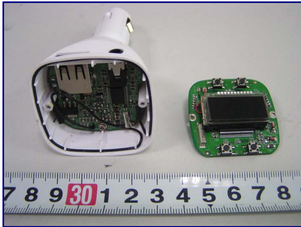
EUT - Uncovered View (3)
