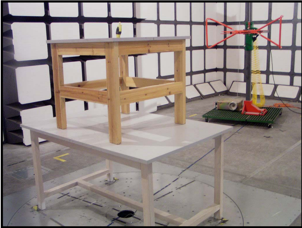
Below 1 GHz: Radiated Emissions-Rear View
