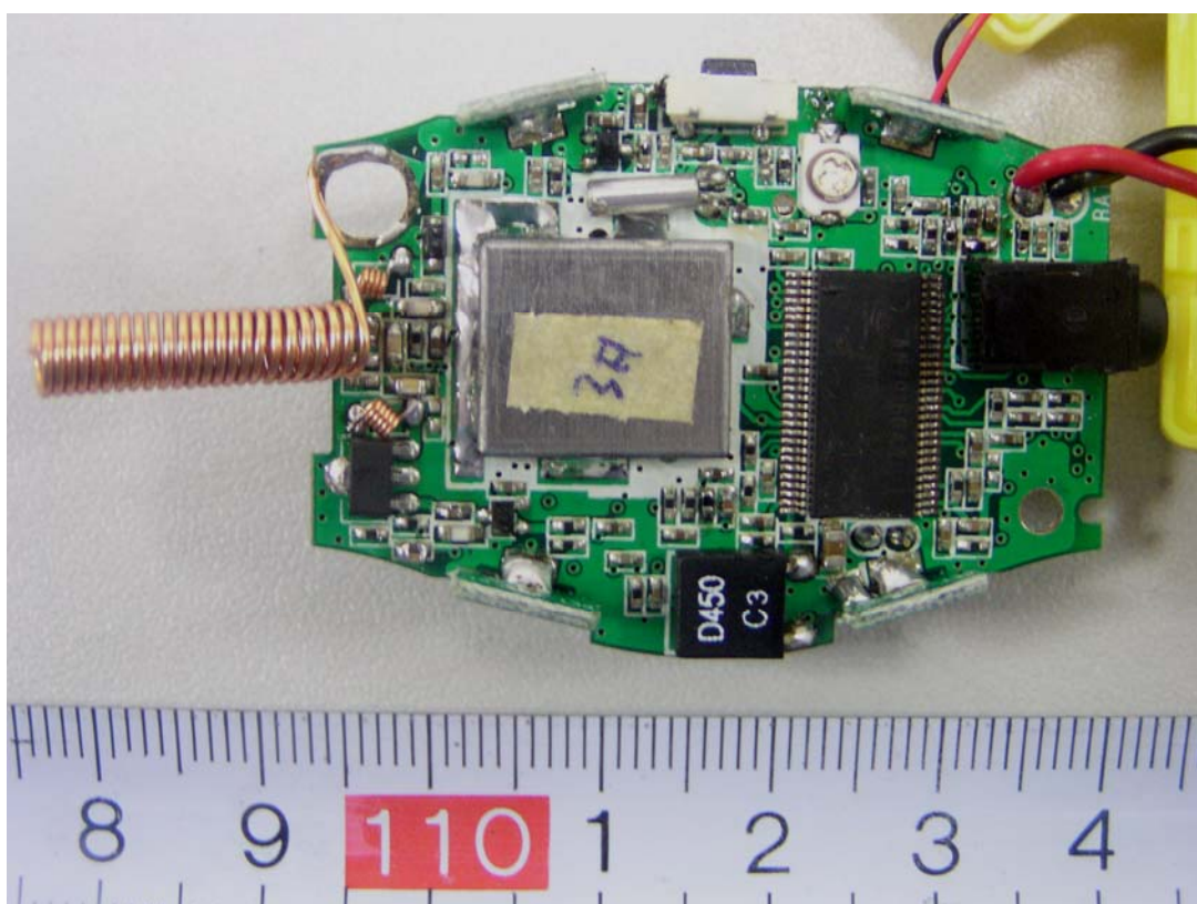
EUT - Board Bottom Components View
