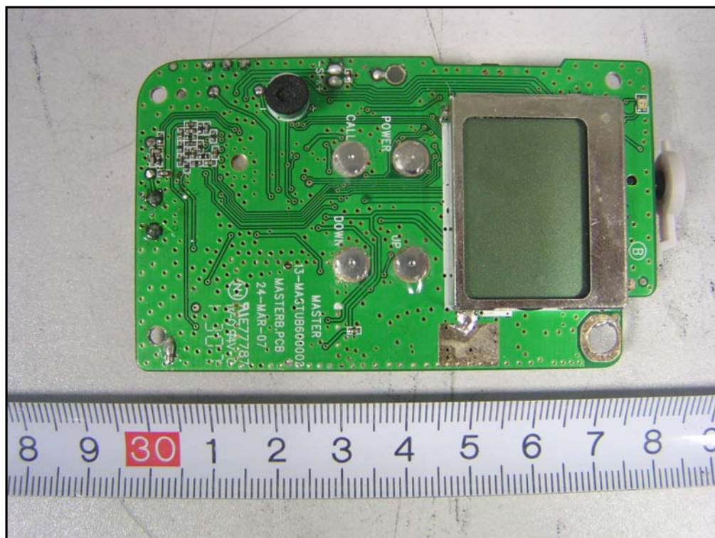
EUT- Board Top Components View
