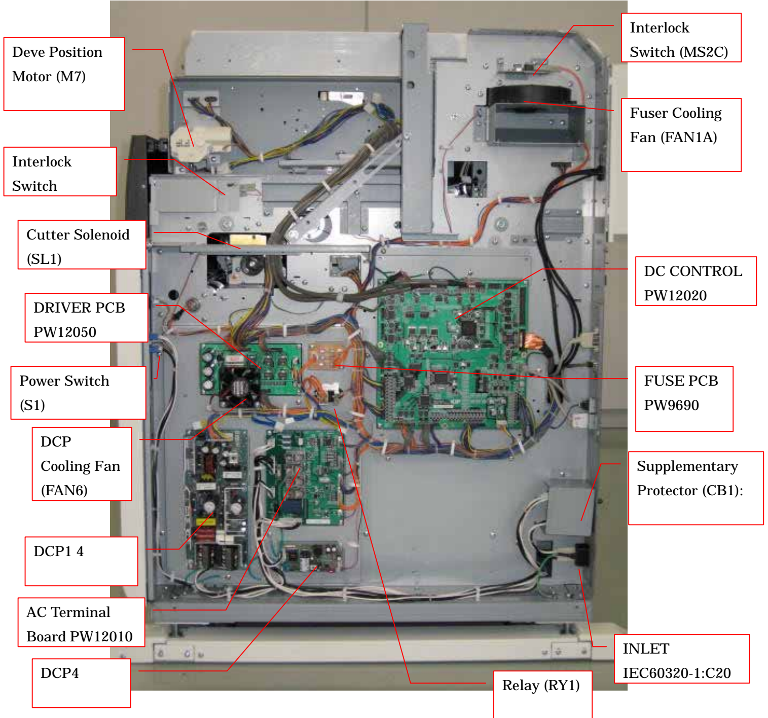
KIP7900 Right side (removed cover)
