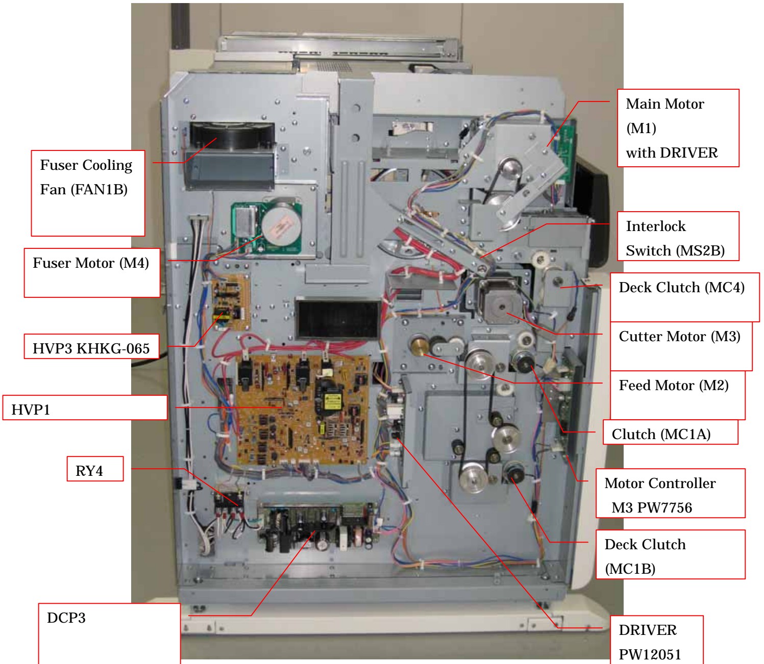
KIP7900 Left side (removed cover)
