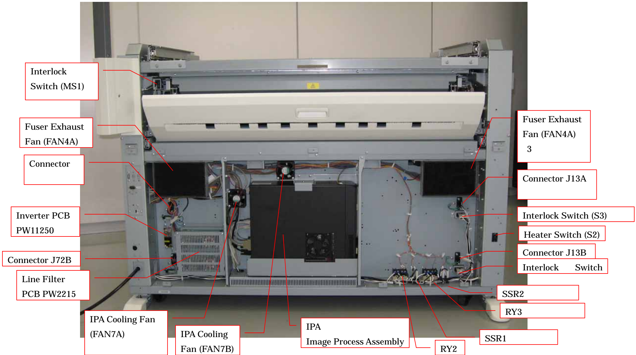
KIP7900 Rear side (removed cover)
