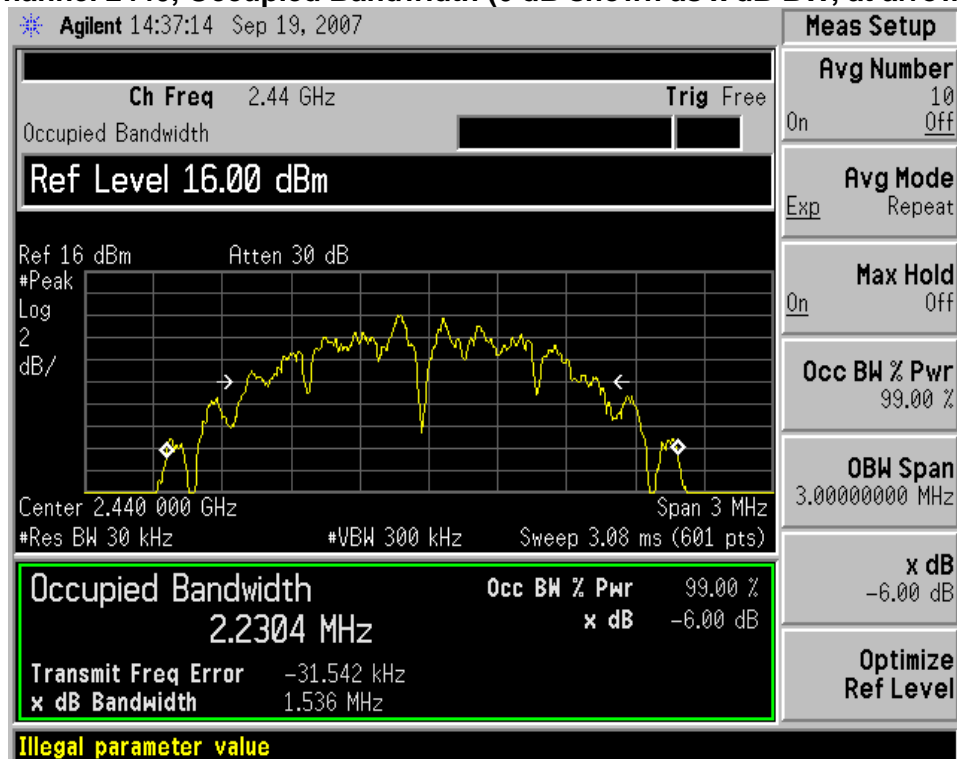
Channel 2440, Occupied Bandwidth (6 dB shown as x dB BW, at arrows)
