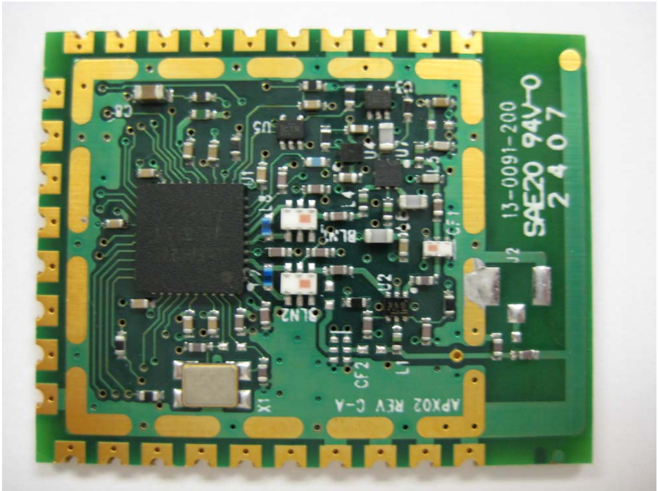
Open for Inspection-View 1
