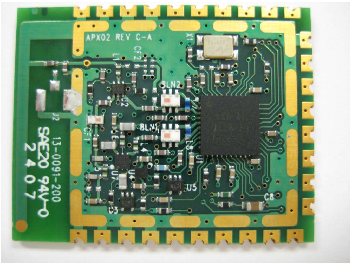
Open for Inspection-View 3, Showing Internal Antenna
