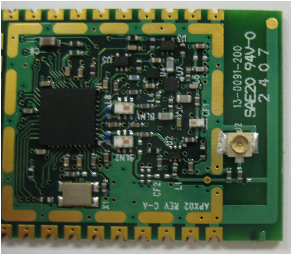
Close-up of Whip Antenna Connector
