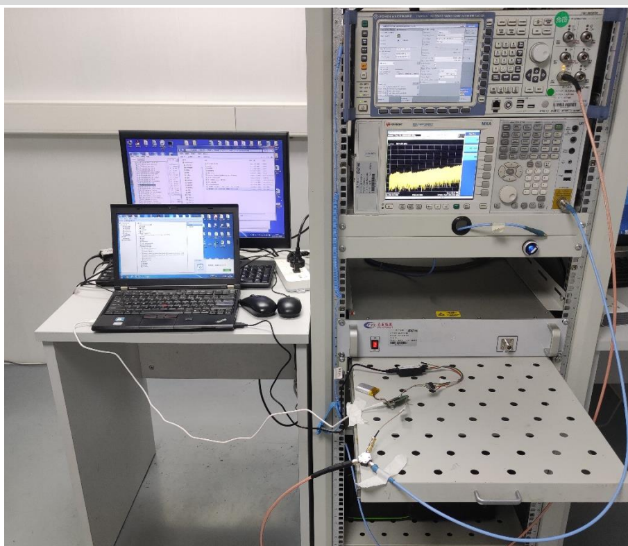
Conducted Test
