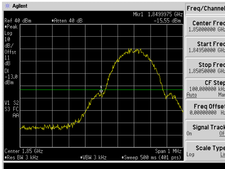
GPRS Lower Channel 512 (1850.2MHz)
