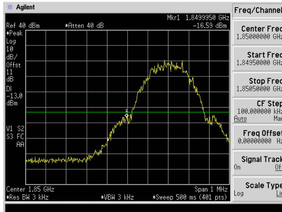
GSM Lower Channel 512 (1850.2MHz)
