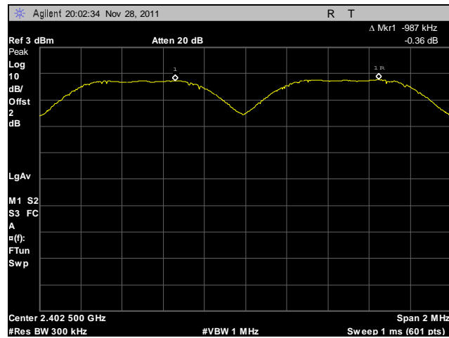
Plot 19. Channel Separation, Channel 0 and 1 (GFSK)
