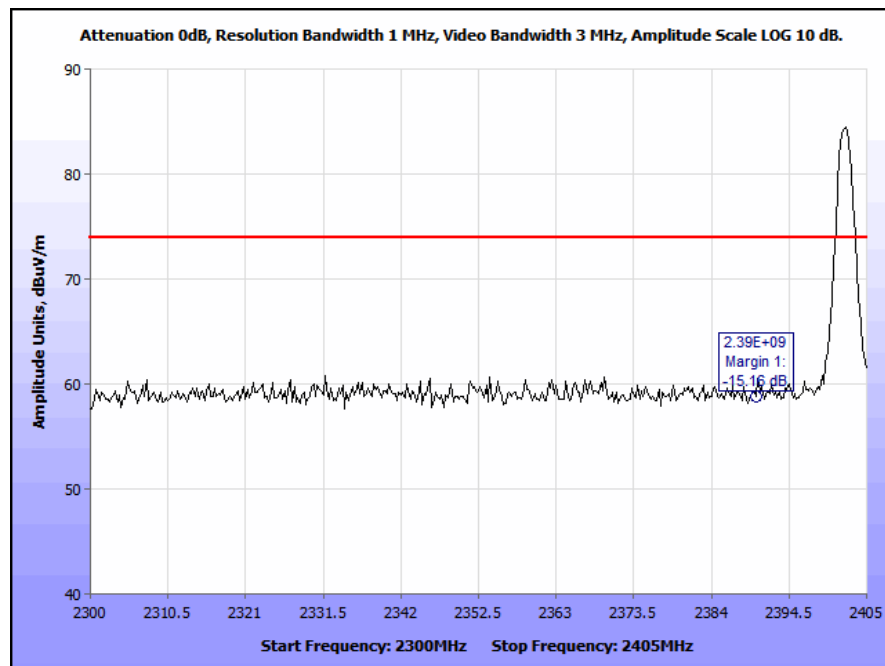
Plot 38. Radiated Restricted Band Edge, Low Channel, Peak
