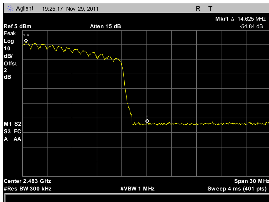
Plot 50. Conducted Band Edge, DPSK, High
