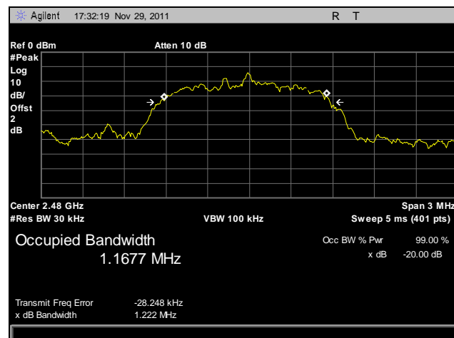
Plot 7. 20 dB Occupied Bandwidth, High Channel, DPSK
