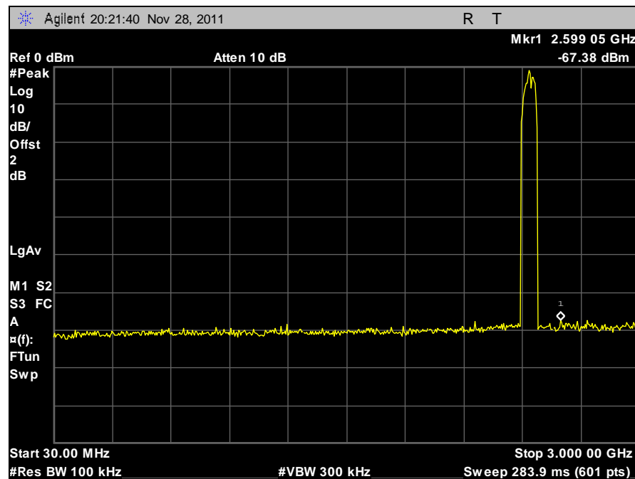
Plot 41. Conducted Spurious Emissions, 30 MHz – 3 GHz, 8PSK
