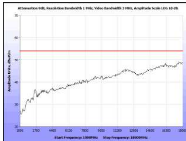
Plot 33. Radiated Spurious Emissions, Mid Channel, Average
