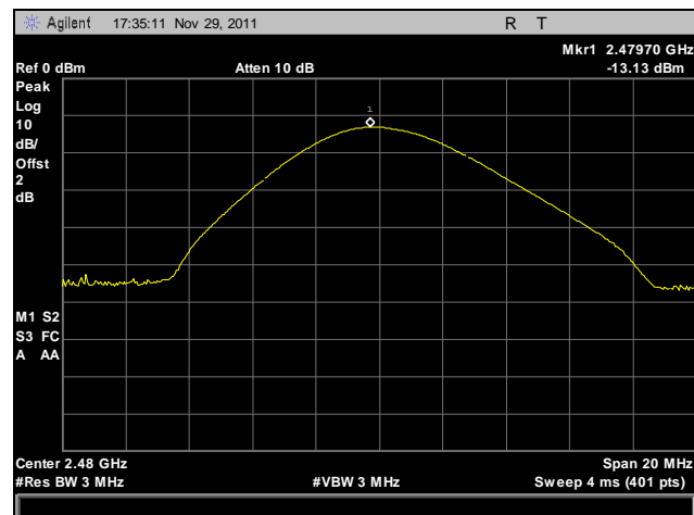
Plot 27. Peak Power Output, High Channel, DPSK
