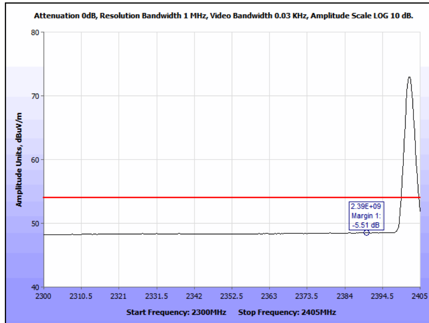
Plot 37. Radiated Restricted Band Edge, Low Channel, Average
