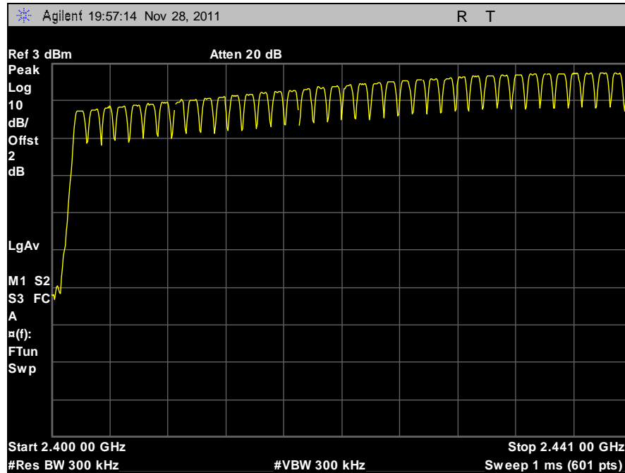
Plot 17. No. of Channels, Chart 1 (2400 – 2441 MHz)
