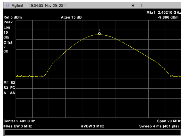
Plot 22. Peak Power Output, Low Channel, 8PSK
