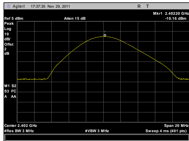
Plot 25. Peak Power Output, Low Channel, DPSK
