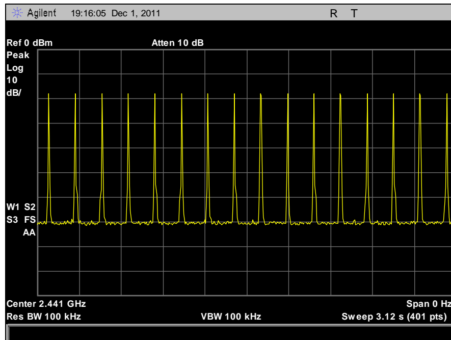
Plot 13. DH3 Burst (16)
