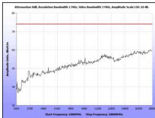
Plot 36. Radiated Spurious Emissions, High Channel, Peak
