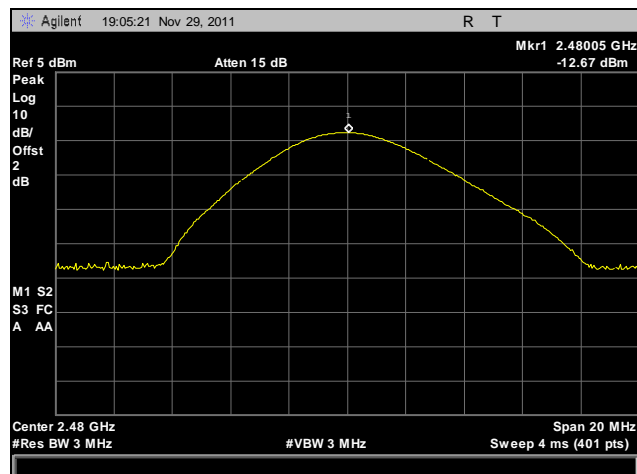
Plot 24. Peak Power Output, High Channel, 8PSK
