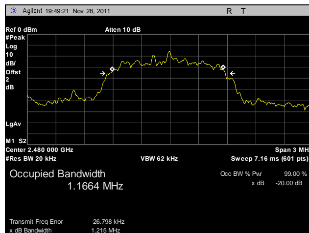
Plot 4. 20 dB Occupied Bandwidth, High Channel, 8 PSK
