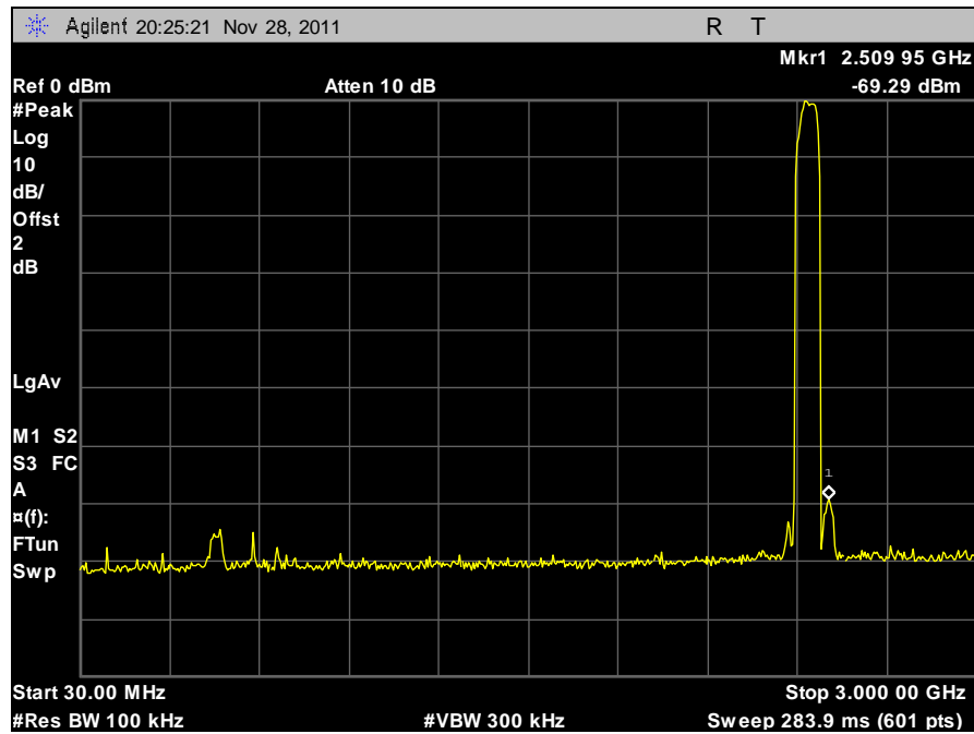
Plot 45. Conducted Spurious Emissions, 30 MHz – 3 GHz, GFSK
