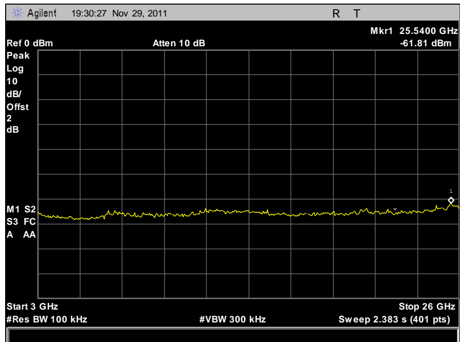
Plot 44. Conducted Spurious Emissions, 3 GHz – 26 GHz, DPSK
