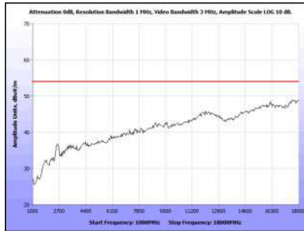
Plot 31. Radiated Spurious Emissions, Low Channel, Average
