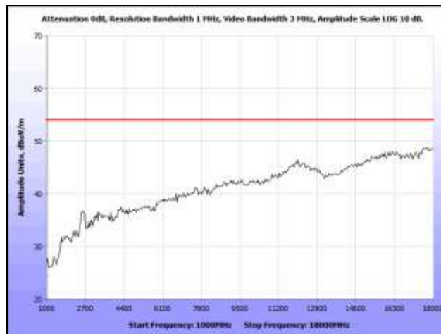
Plot 35. Radiated Spurious Emissions, High Channel, Average
