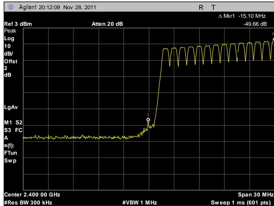
Plot 51. Conducted Band Edge, GFSK, Low
