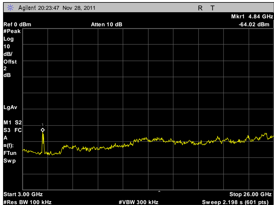
Plot 46. Conducted Spurious Emissions, 3 GHz – 26 GHz, GFSK
