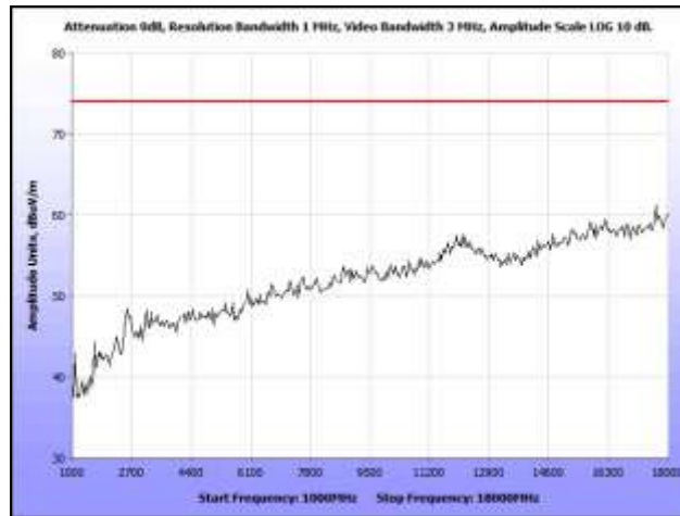
Plot 34. Radiated Spurious Emissions, Mid Channel, Peak
