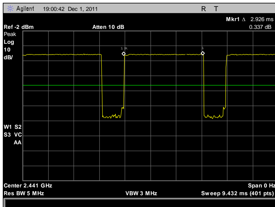
Plot 16. DH5 on Time
