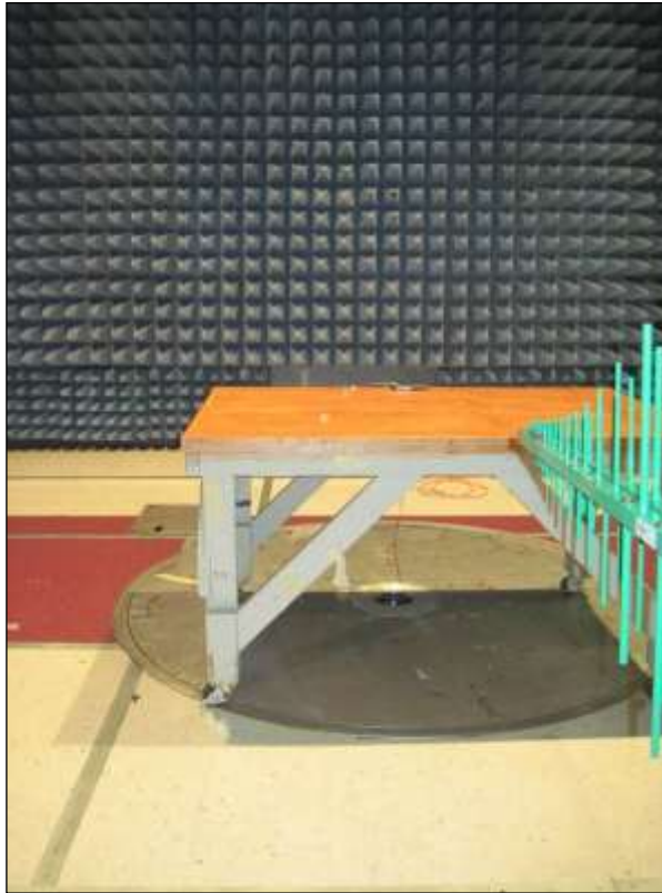
Photograph 2. Radiated Emissions, Test Setup, Antenna View
