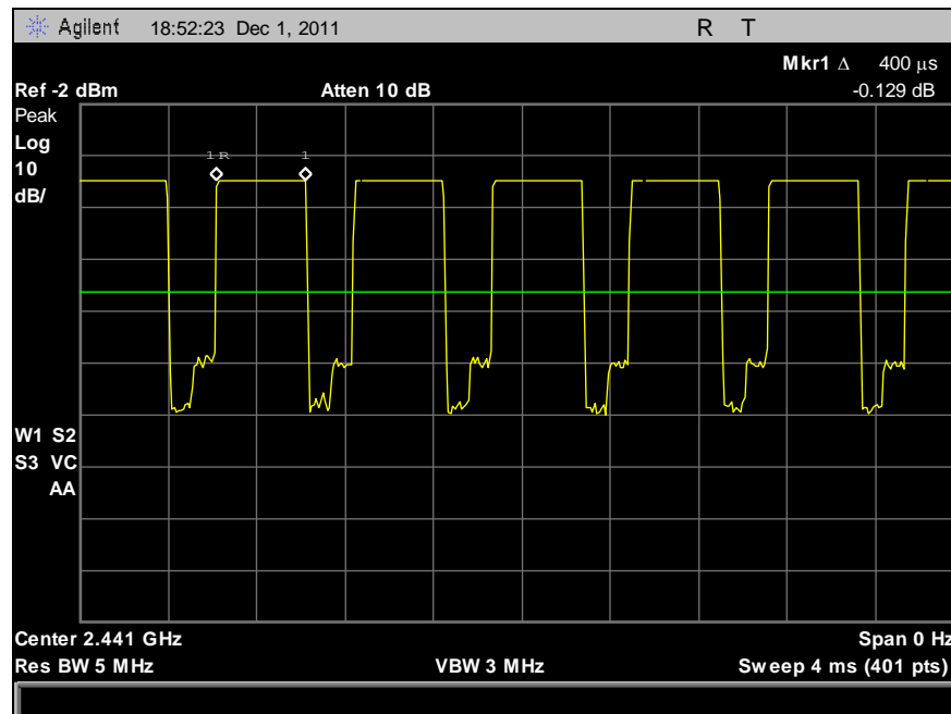
Plot 12. DH1 on Time
