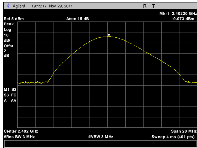
Plot 28. Peak Power Output, Low Channel, GFSK
