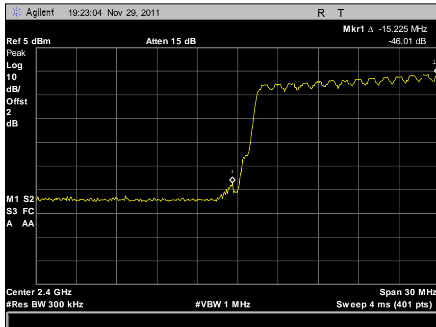
Plot 49. Conducted Band Edge, DPSK, Low
