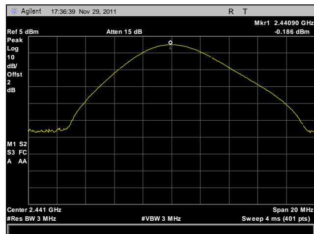
Plot 26. Peak Power Output, Mid Channel, DPSK
