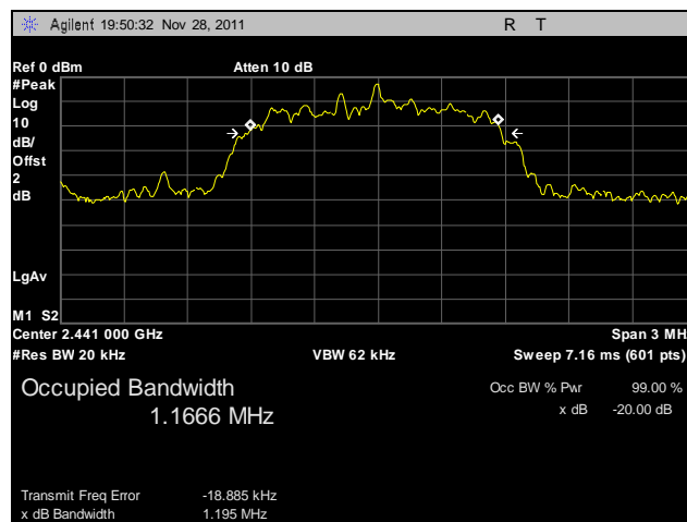
Plot 3. 20 dB Occupied Bandwidth, Mid Channel, 8 PSK
