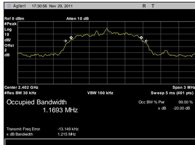
Plot 5. 20 dB Occupied Bandwidth, Low Channel, DPSK
