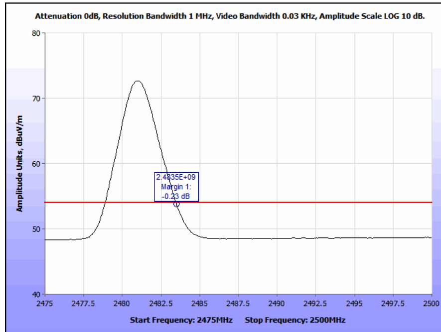
Plot 39. Radiated Restricted Band Edge, High Channel, Average
