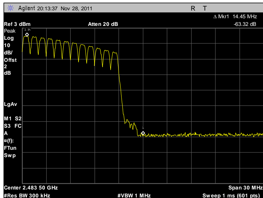
Plot 52. Conducted Band Edge, GFSK, High
