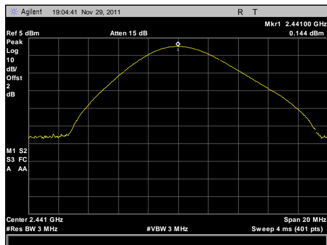
Plot 23. Peak Power Output, Mid Channel, 8PSK
