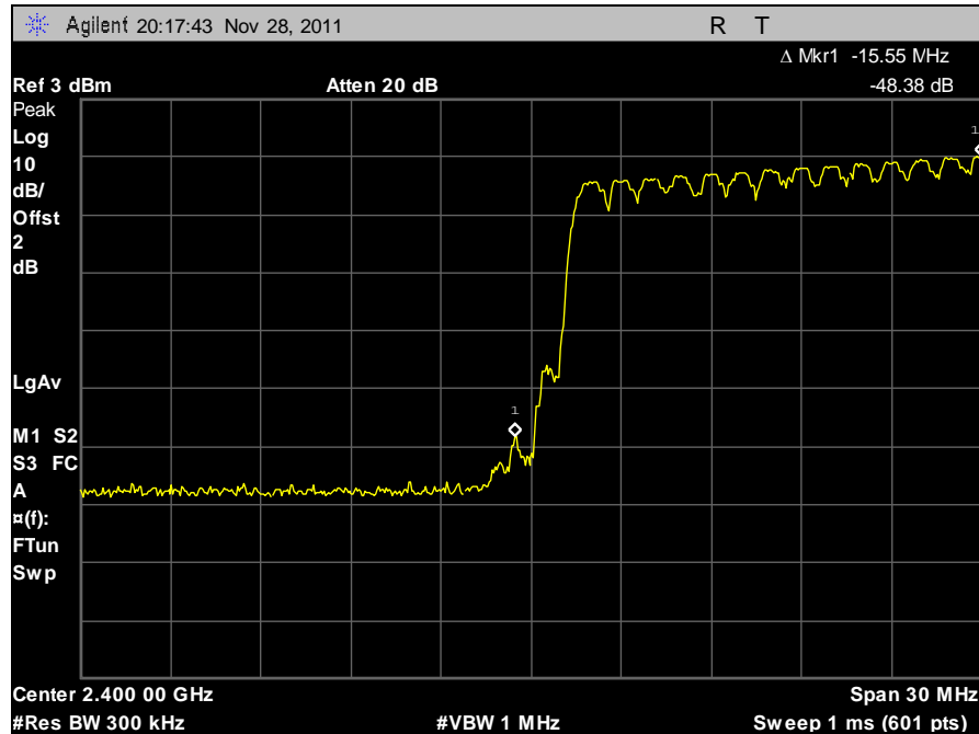
Plot 47. Conducted Band Edge, 8PSK, Low
