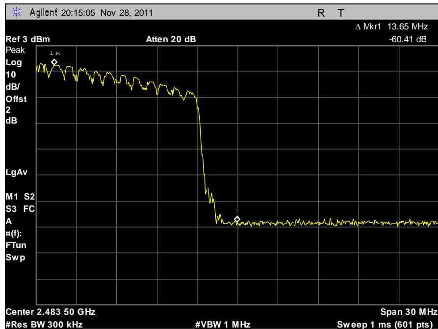
Plot 48. Conducted Band Edge, 8PSK, High
