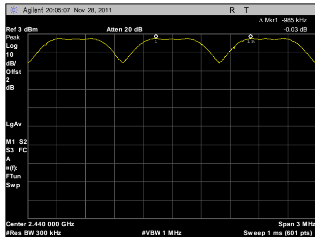
Plot 20. Channel Separation, Channel 39 and 40 (GFSK)
