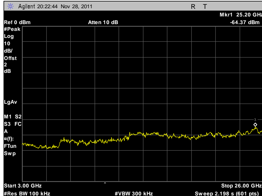
Plot 42. Conducted Spurious Emissions, 3 GHz – 26 GHz, 8PSK
