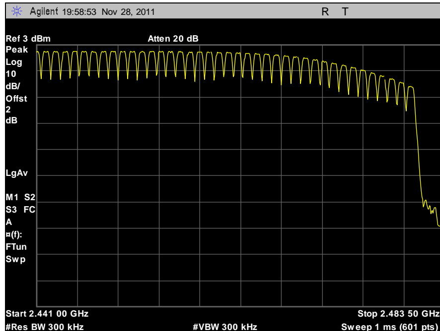
Plot 18. No. of Channels, Chart 2 (2441 – 2483.5 MHz)
