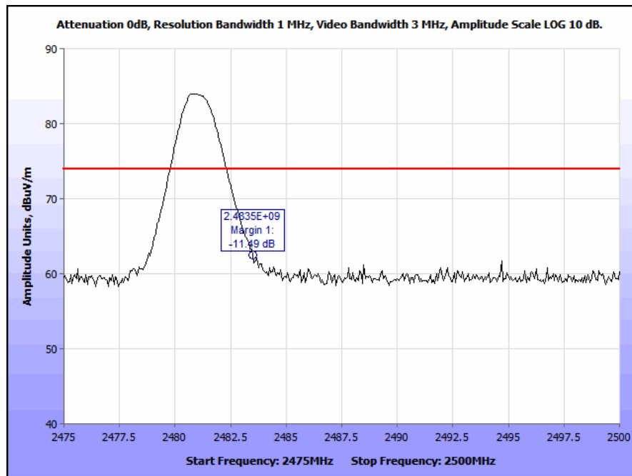
Plot 40. Radiated Restricted Band Edge, High Channel, Peak
