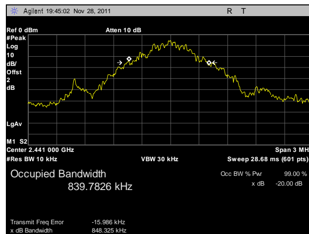
Plot 9. 20 dB Occupied Bandwidth, Mid Channel, GFSK
