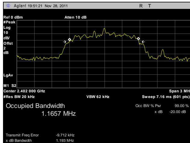
Plot 2. 20 dB Occupied Bandwidth, Low Channel, 8 PSK
