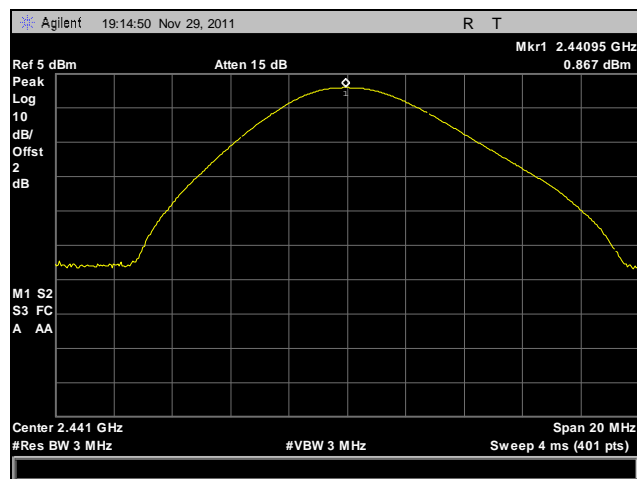
Plot 29. Peak Power Output, Mid Channel, GFSK
