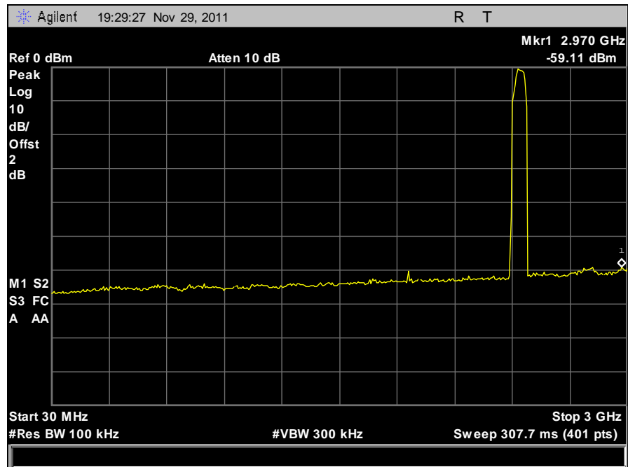
Plot 43. Conducted Spurious Emissions, 30 MHz – 3 GHz, DPSK
