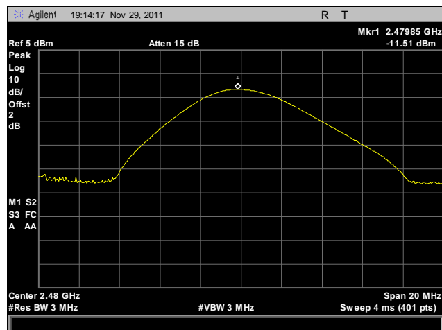
Plot 30. Peak Power Output, High Channel, GFSK
