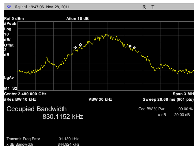
Plot 10. 20 dB Occupied Bandwidth, High Channel, GFSK
