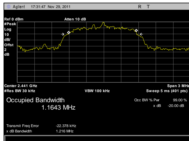
Plot 6. 20 dB Occupied Bandwidth, Mid Channel, DPSK
