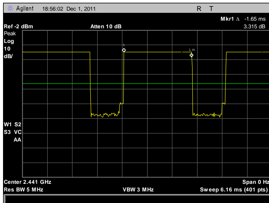
Plot 14. DH3 on Time
