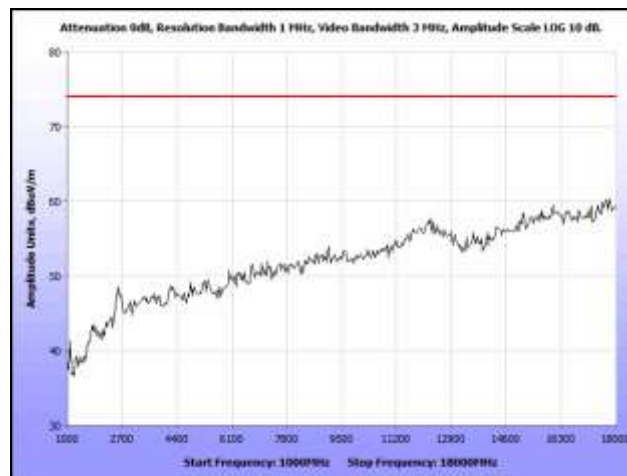
Plot 32. Radiated Spurious Emissions, Low Channel, Peak
