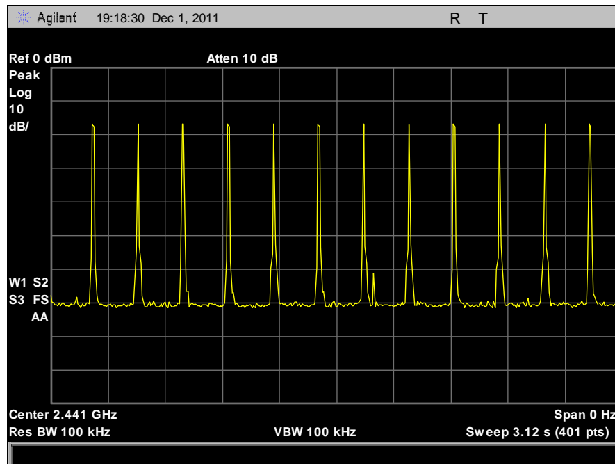
Plot 15. DH5 Burst (12)
