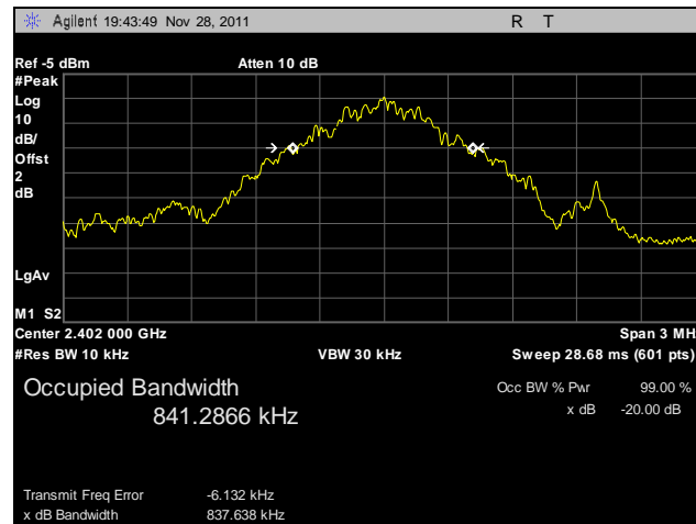
Plot 8. 20 dB Occupied Bandwidth, Low Channel, GFSK
