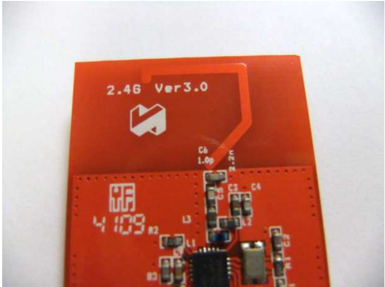
Photo 4 Close-Up of PCB Antenna embedded in PCB
