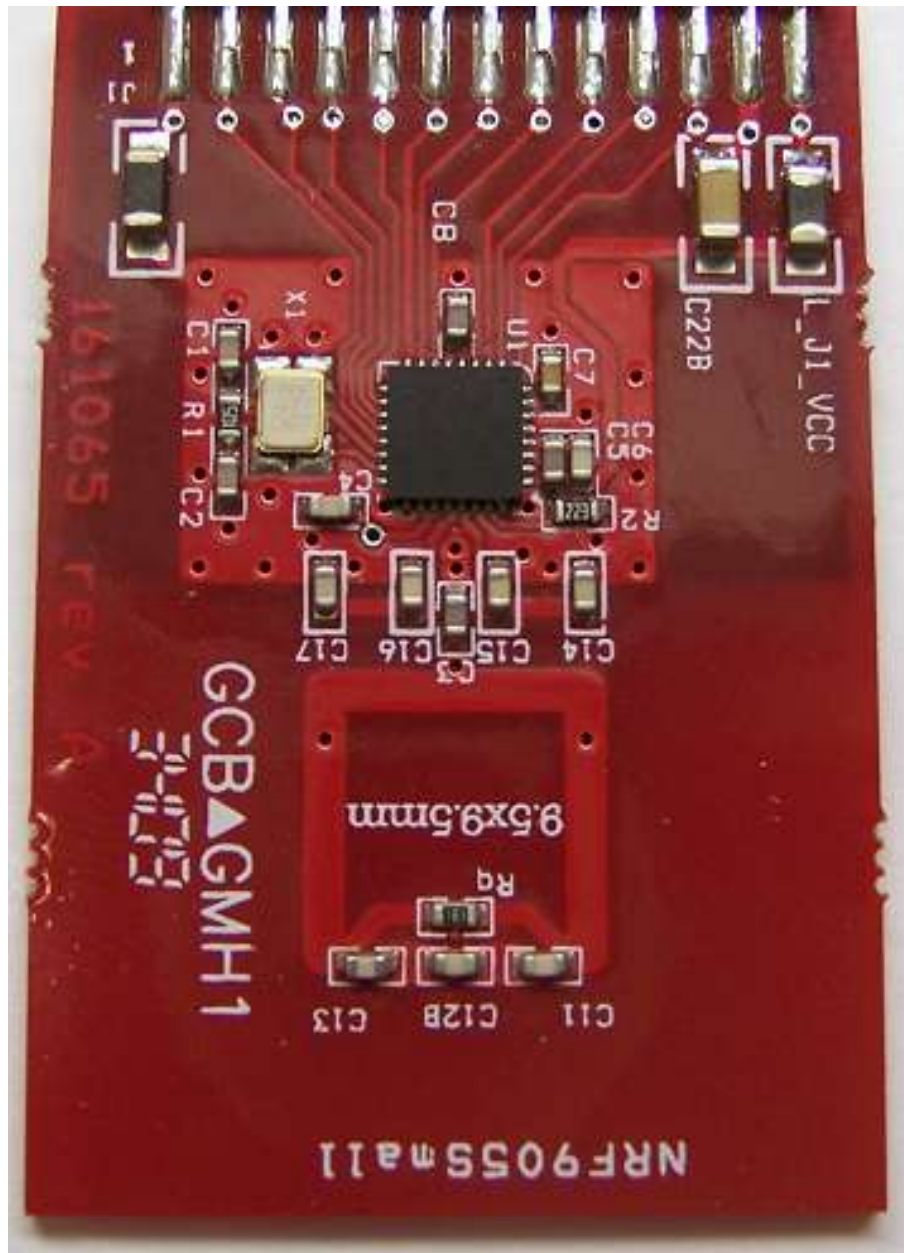
Photo 4 Close-Up of PCB Antenna embedded in PCB
