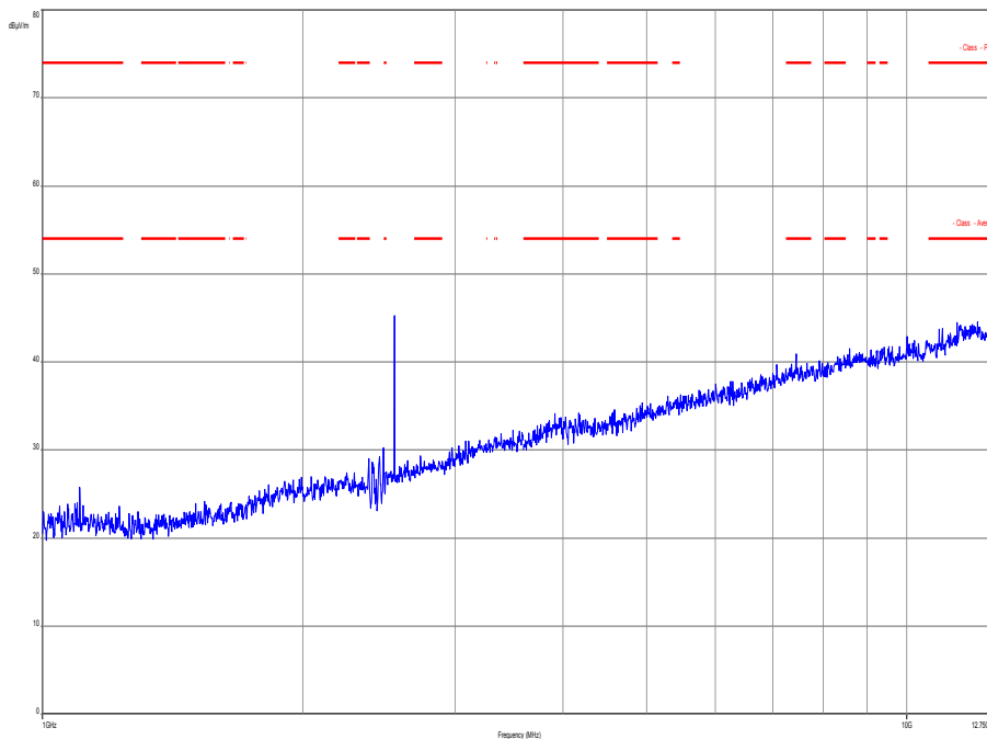
Plot 7: 1 GHz to 12.75 GHz, TX mode, channel 39, vertical & horizontal polarization
