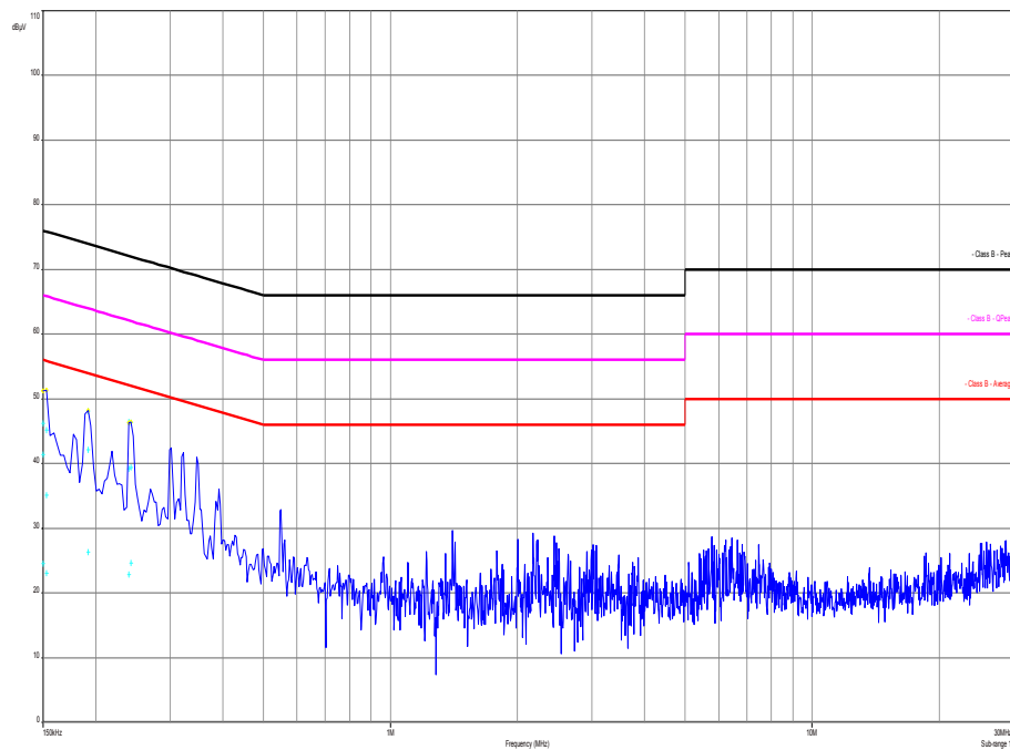
Plot 4: 150 kHz to 30 MHz, RX mode, neutral line
