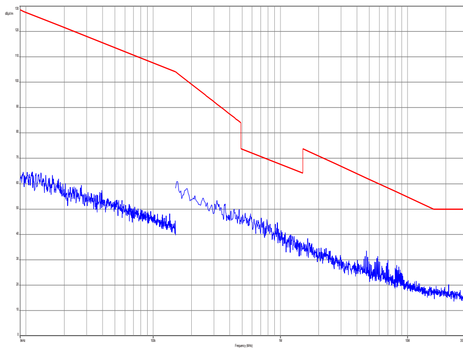
Plot 3: 9 kHz to 30 MHz, channel 39, transmit mode
