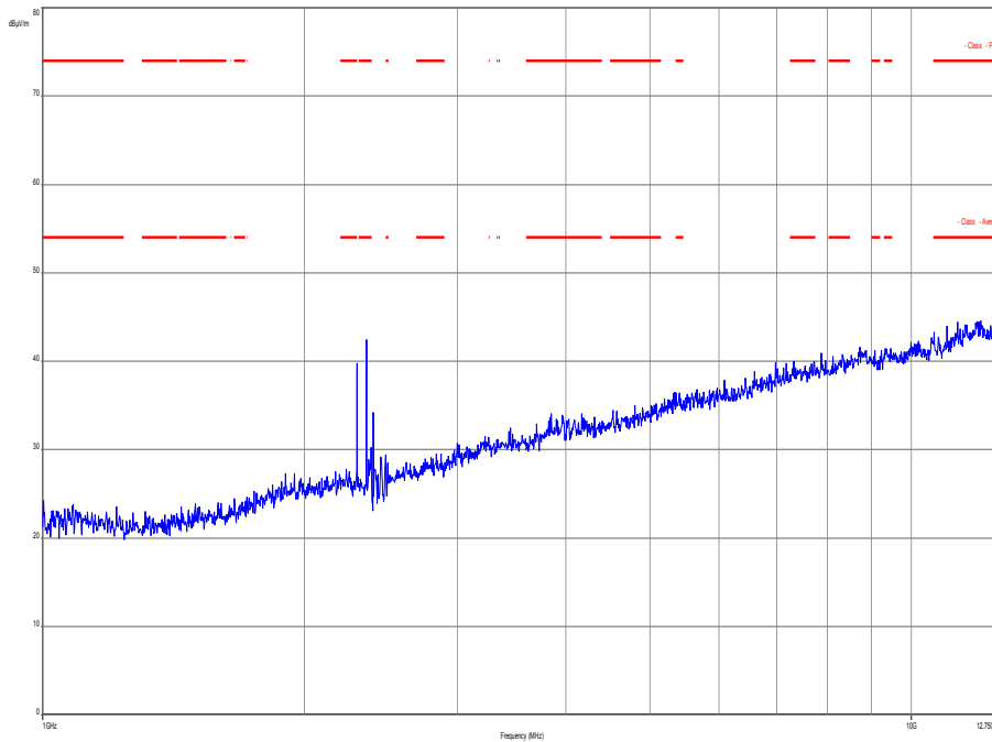
Plot 1: 1 GHz to 12.75 GHz, TX mode, channel 00, vertical & horizontal polarization
