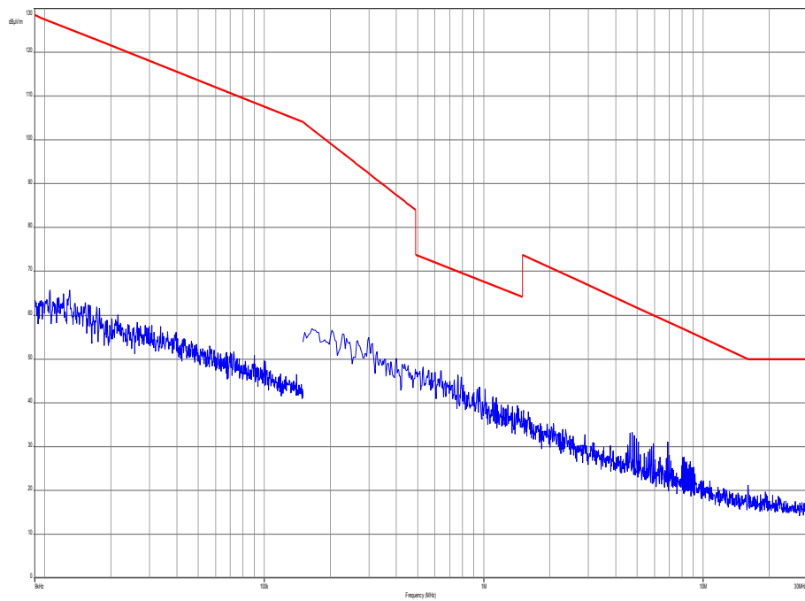
Plot 2: 9 kHz to 30 MHz, channel 19, transmit mode
