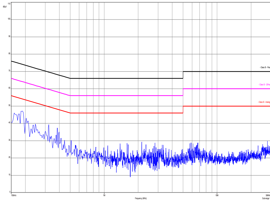
Plot 2: 150 kHz to 30 MHz, TX mode, neutral line
