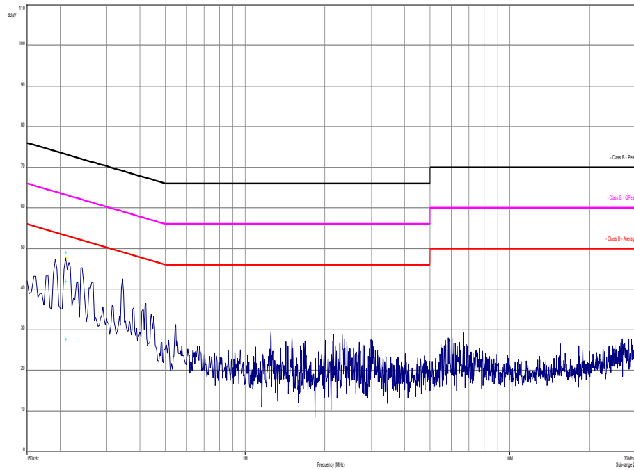
Plot 3: 150 kHz to 30 MHz, RX mode, phase line
