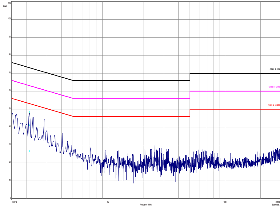
Plot 1: 150 kHz to 30 MHz, TX mode, phase line
