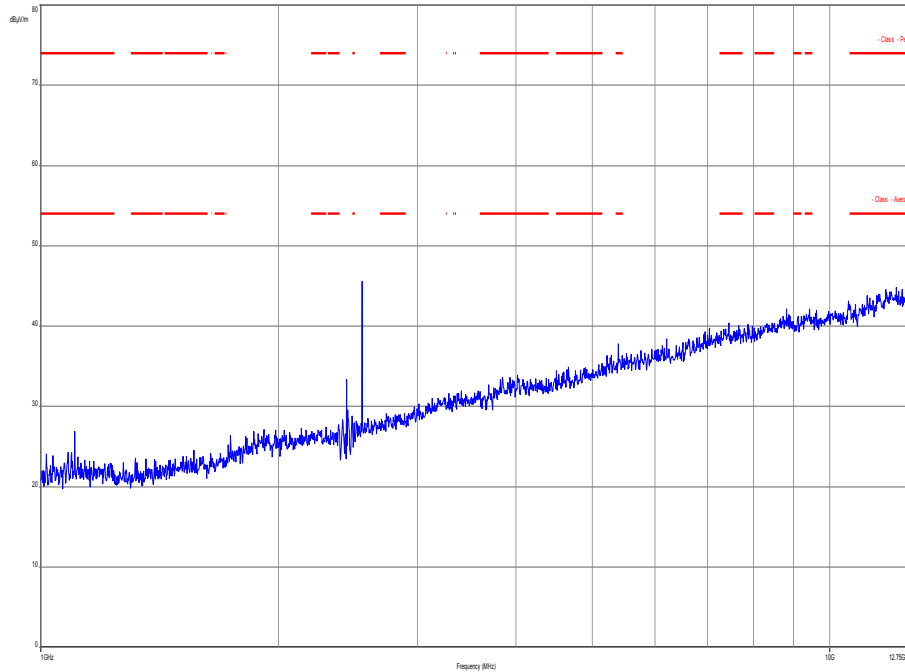
Plot 4: 1 GHz to 12.75 GHz, TX mode, channel 19, vertical & horizontal polarization
