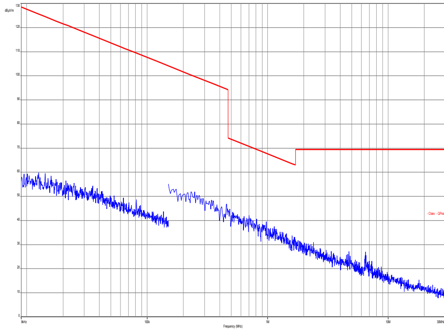
Plot 1: 9 kHz to 30 MHz, channel 00, transmit mode
