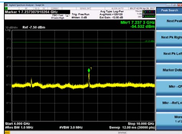
802.11n – 4-10 GHz – Low Channel
