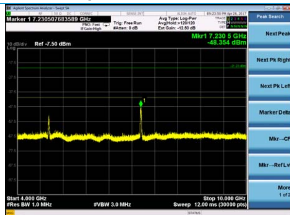
802.11g – 4-10 GHz – Low Channel
