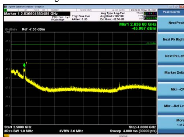
802.11g – 2.5-4 GHz – Low Channel
