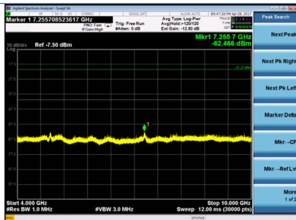
802.11n HT-40 – 4-10 GHz – Low Channel
