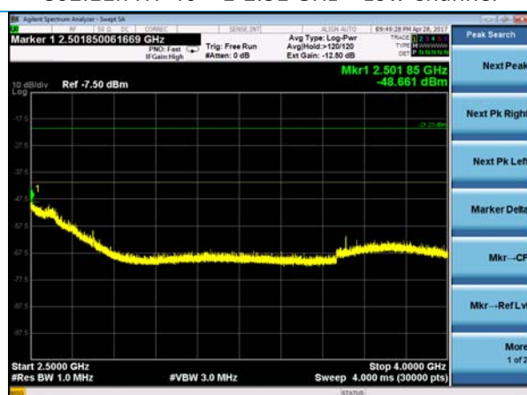
802.11n HT-40 – 2.5-4 GHz – Low Channel
