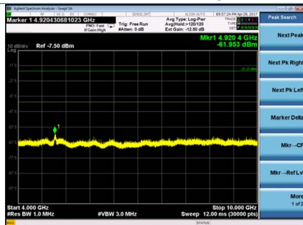
802.11n HT-40 – 4-10 GHz – High Channel
