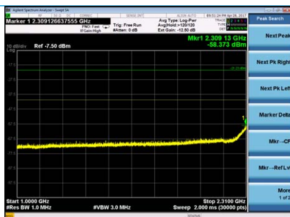
802.11n HT-40 – 1-2.31 GHz – Low Channel
