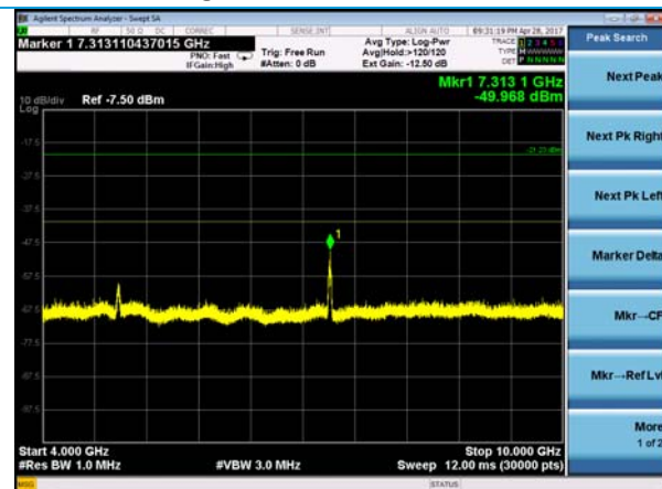
802.11g – 4-10 GHz – Mid Channel
