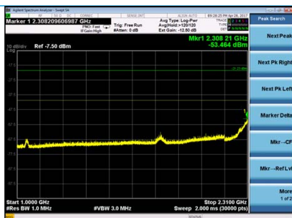
802.11g- 1-2.31 GHz – Low Channel
